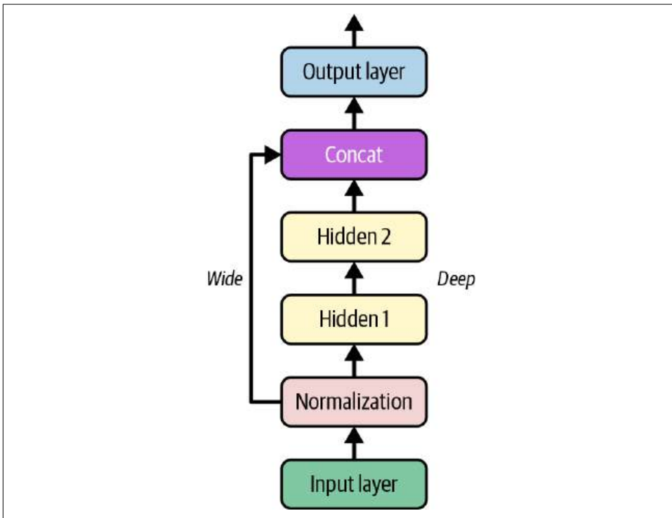
Figure 10-13. Wide & Deep neural network
