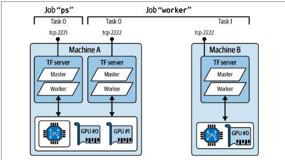
Figure 19-18. An example TensorFlow cluster
