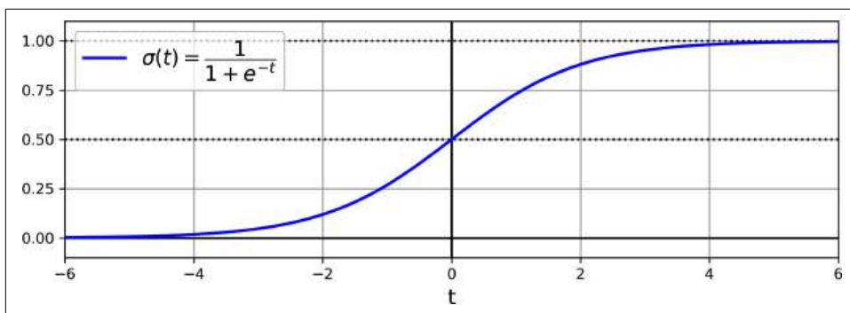
Figure 4-21. Logistic function
