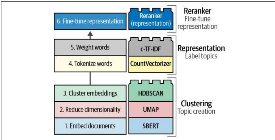
Figure 5-20. The reranker (representation) block sits on top of the c-TF-IDF representation.
