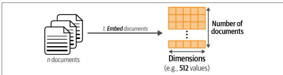
Figure 5-3. Step 1: We convert documents to embeddings using an embedding model.
