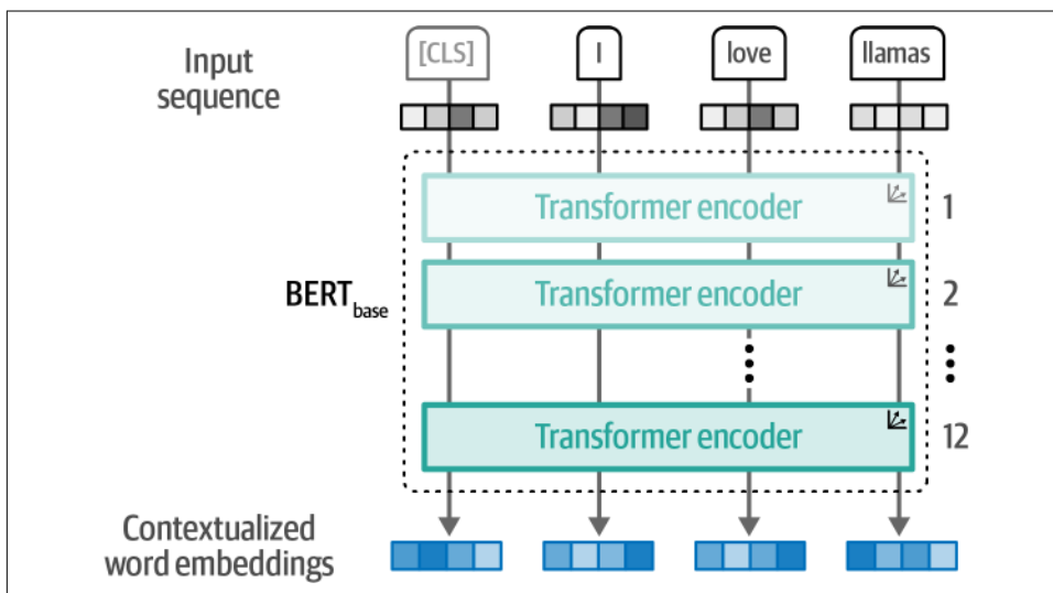
Figure 1-21. The architecture of a BERT base model with 12 encoders.
