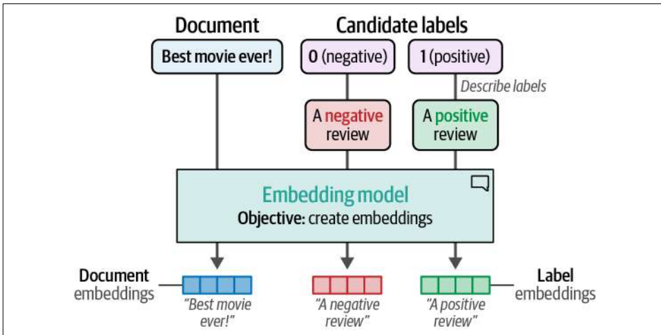
Figure 4-14. To embed the labels, we first need to give them a description, such as “a negative movie review.” This can then be embedded through sentence-transformers.
