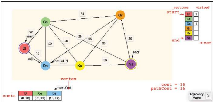
FIGURE 15-16 After selecting Da(hl) to visit in finding the shortest path to Naur
