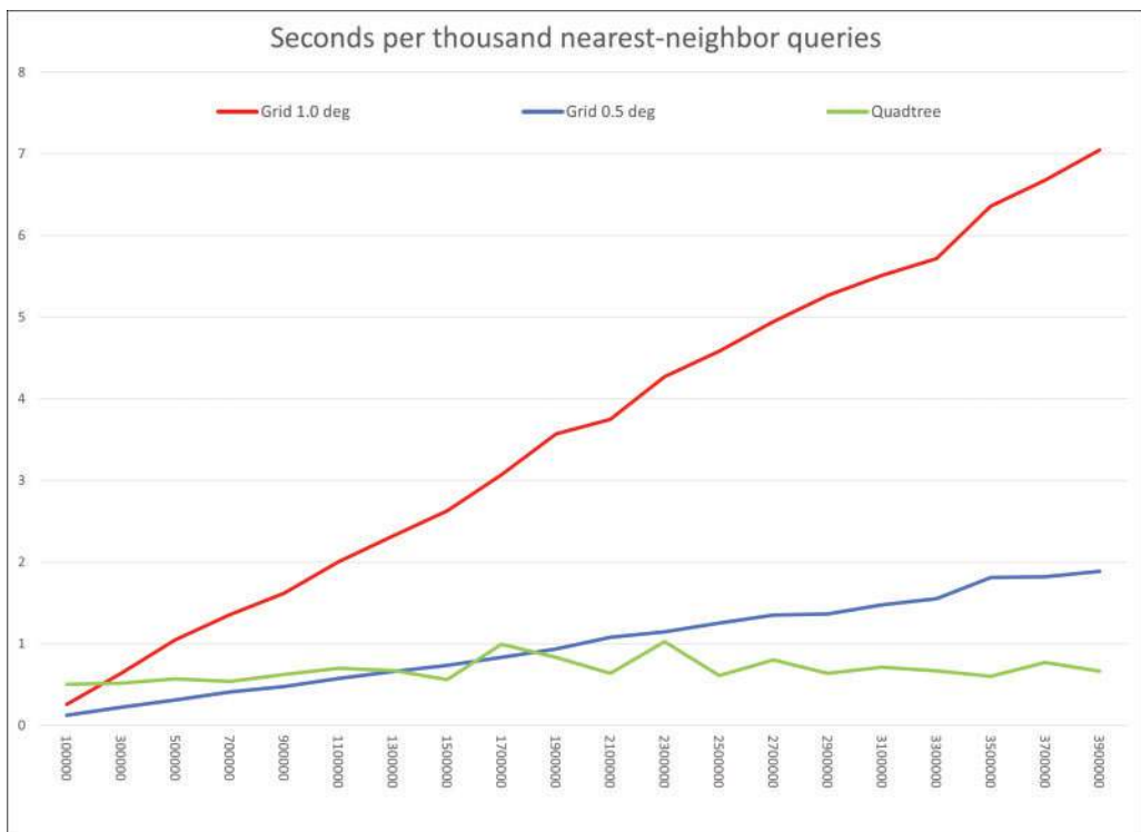
FIGURE 12-30 Performance of findNearest() on different-sized data sets
