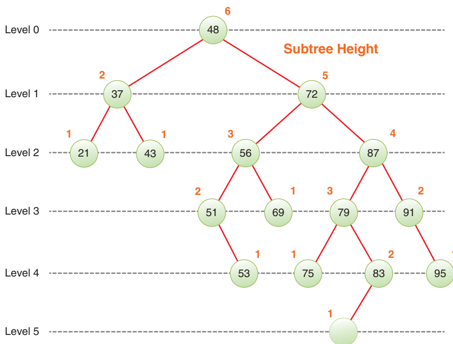
FIGURE 10-5 Node levels and subtree heights
