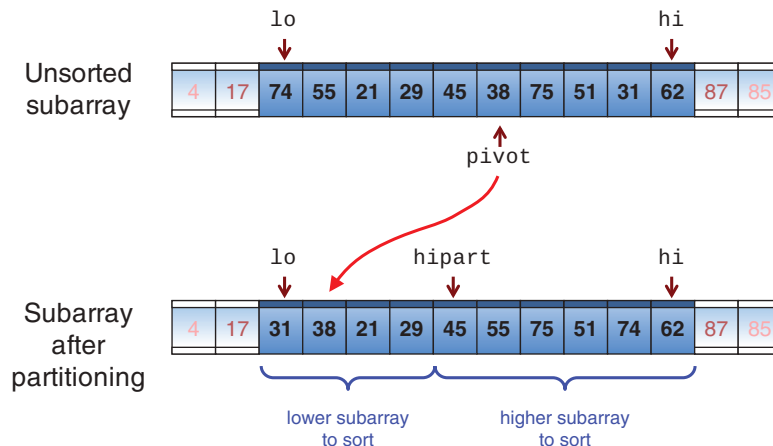
FIGURE 7-7 Partitioning in one call to quicksort_sketch()
