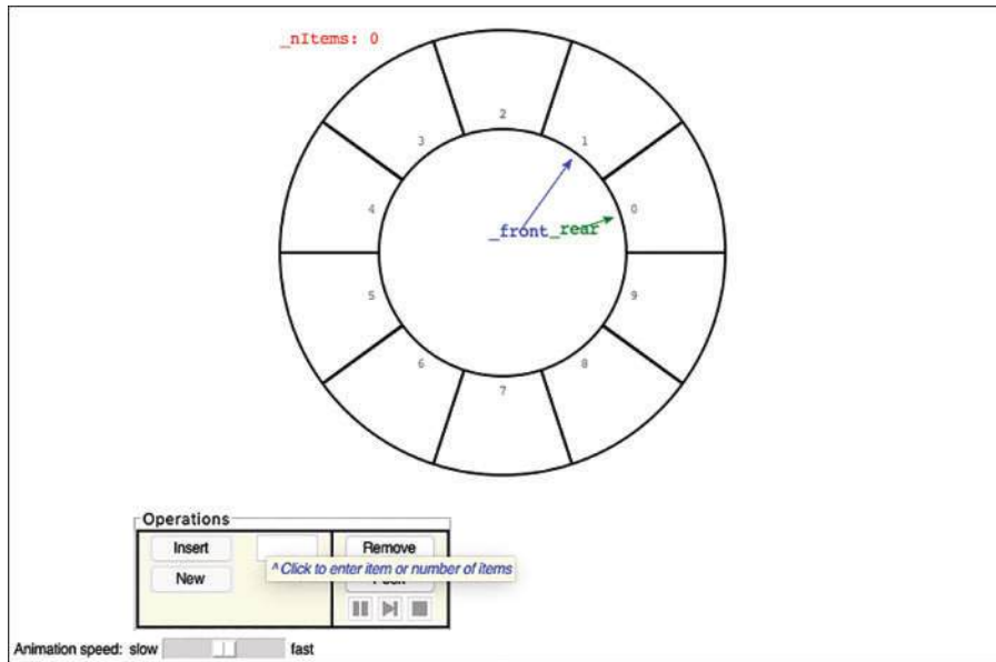
FIGURE 4-6 The Queue Visualization tool
