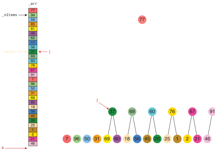
FIGURE 13-13 Heapifying an array of 30 random items in the Visualization tool Humble Bundle Pearson Python Bundle – © Pearson. Do Not Distribute.
