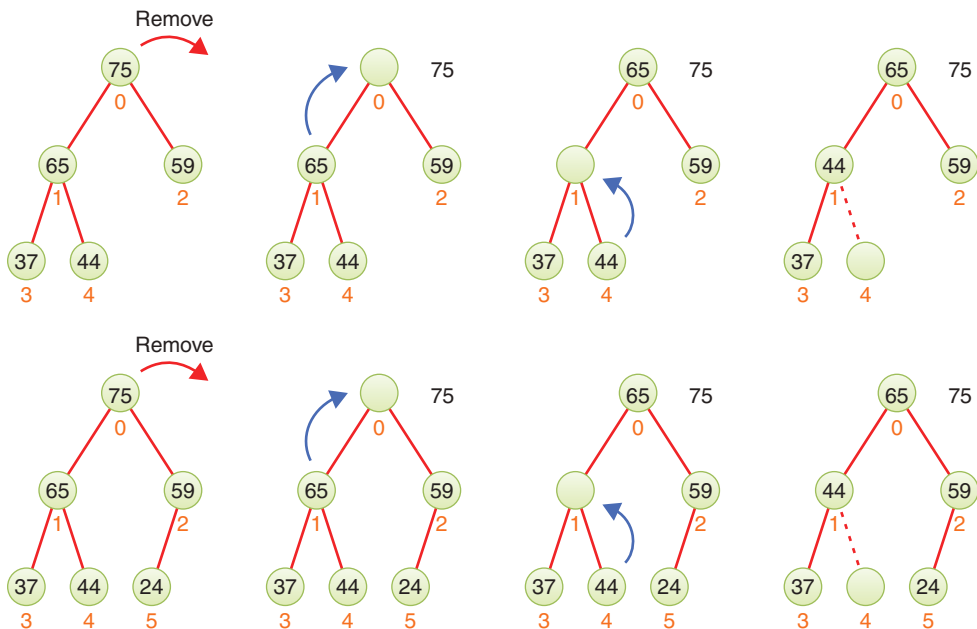
FIGURE 13-4 Two examples of filling holes with the maximum child item
