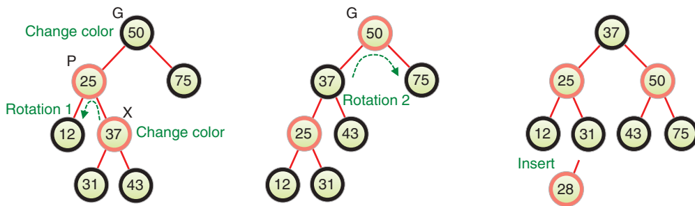
FIGURE 10-30 Correcting a red-red inside grandchild on the way down
