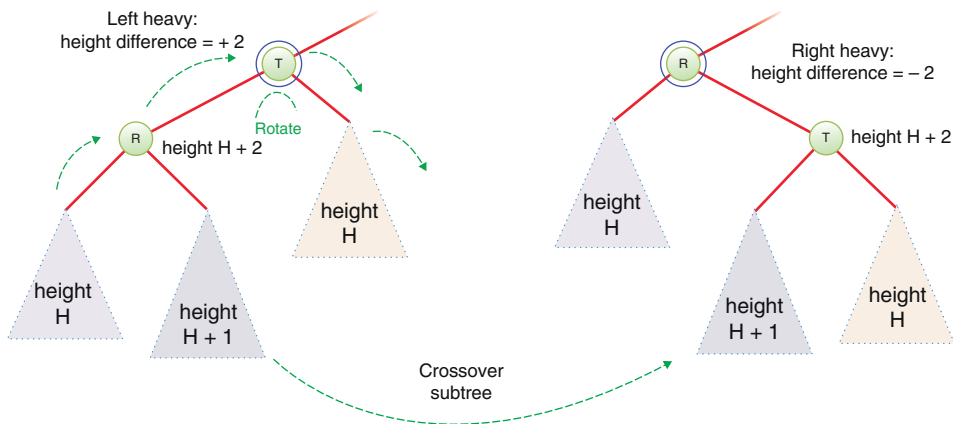
FIGURE 10-13 Balancing a left-heavy subtree
