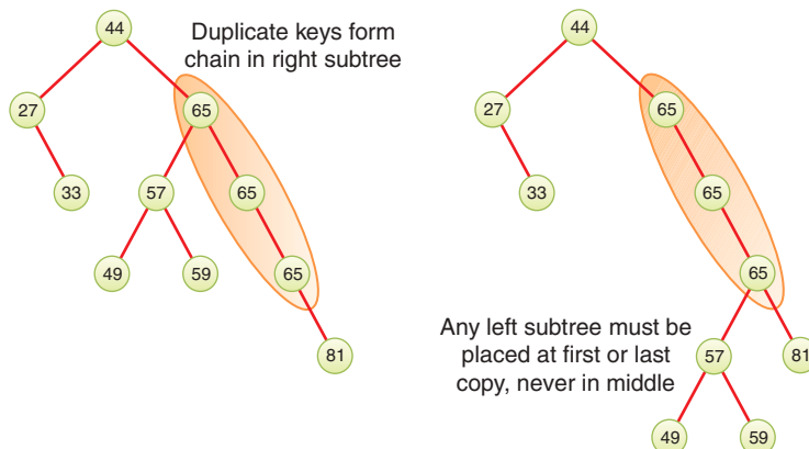
FIGURE 8-26 Duplicate keys in binary search trees
