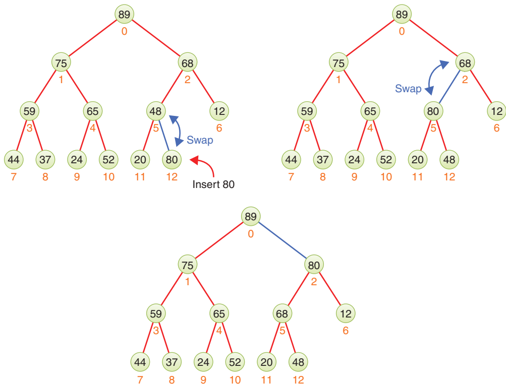
FIGURE 13-3 Inserting an item in a heap and sifting up
