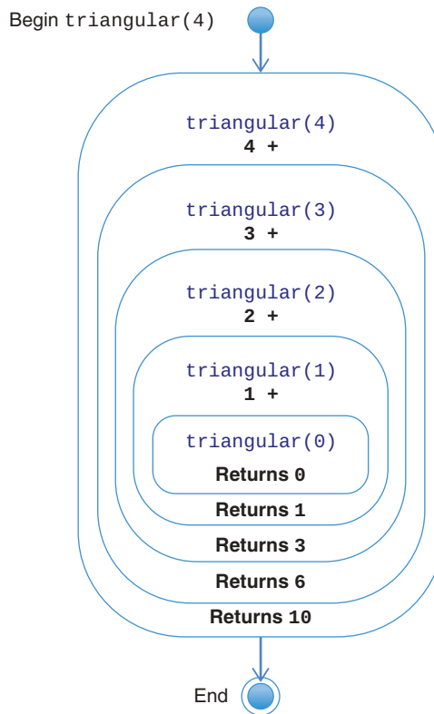
FIGURE 6-5 Execution of the recursive triangular(4) function
