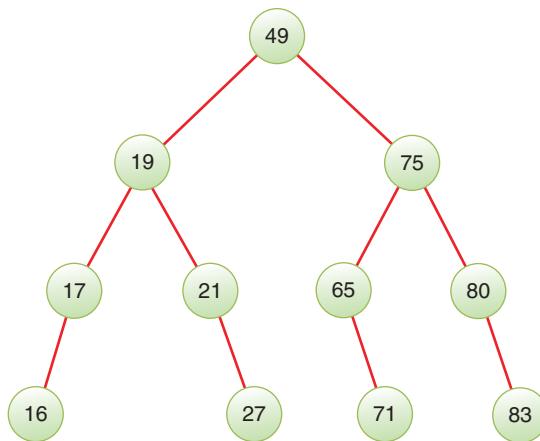
FIGURE 10-4 A nearly symmetric, balanced binary tree
