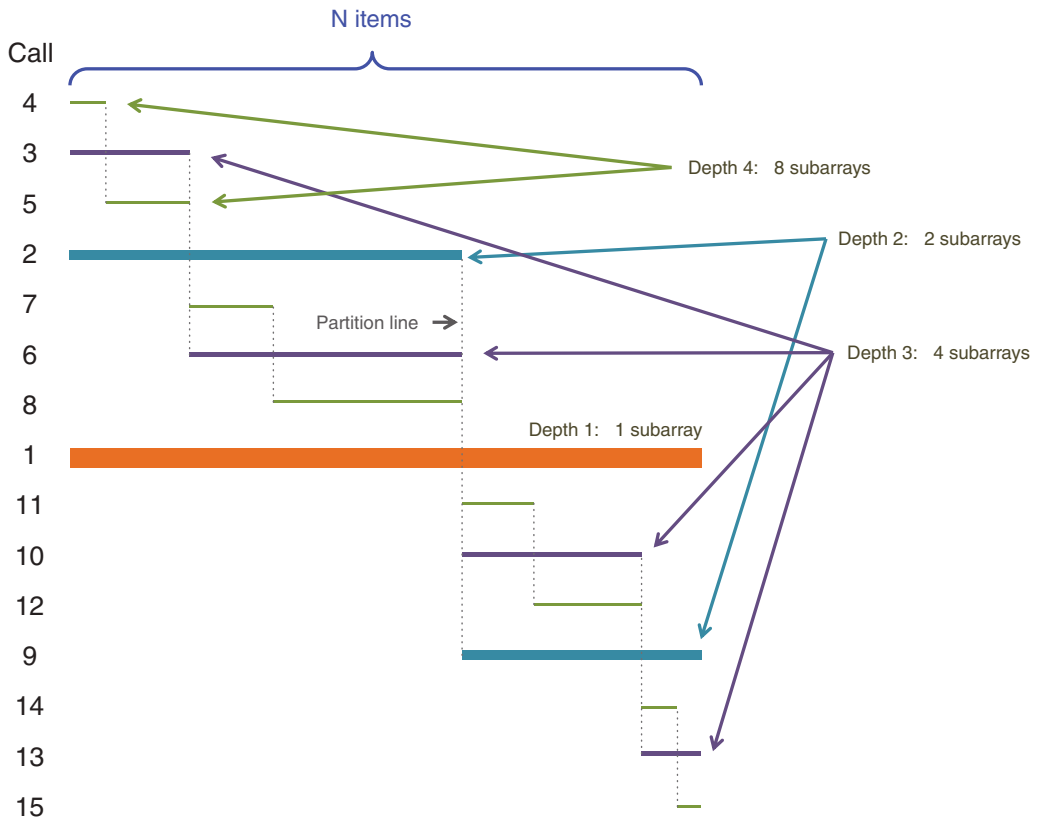
FIGURE 7-15 Lines corresponding to partitions in quicksort
