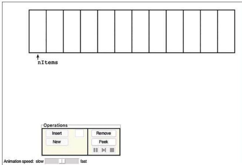
FIGURE 4-10 The PriorityQueue Visualization tool
