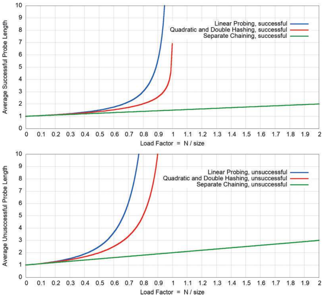
FIGURE 11-20 Successful and unsuccessful probe performance
