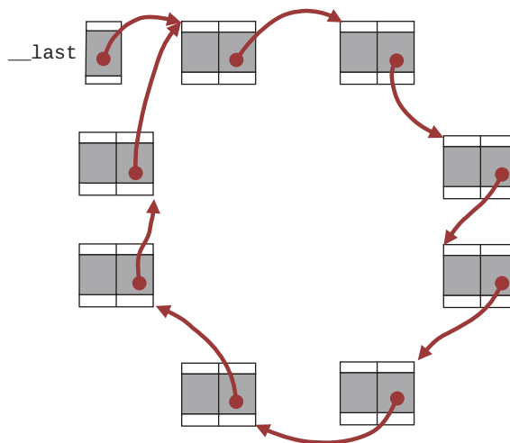
FIGURE 5-14 A circular linked list (without data)
