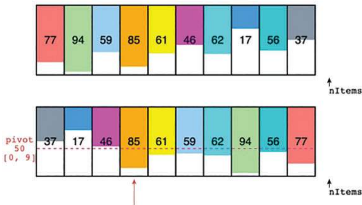
FIGURE 7-6 Partitioning a 10-element array in the AdvancedSorting Visualization tool
