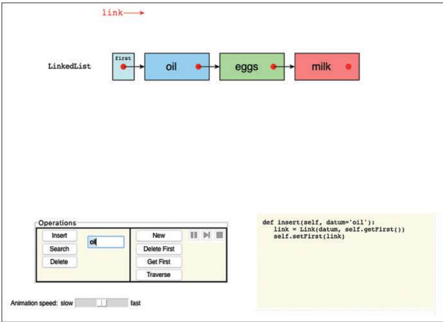
FIGURE 5-4 A linked list after inserting some items
