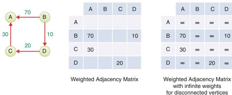
FIGURE 15-19 A weighted, directed graph and its adjacency matrix Humble Bundle Pearson Python Bundle – © Pearson. Do Not Distribute.
