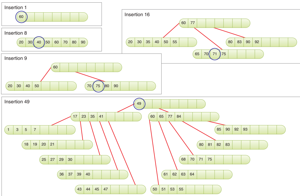
FIGURE 9-21 Building a B-tree
