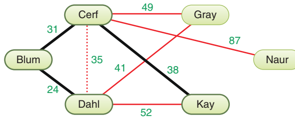
FIGURE 15-7 The minimum spanning tree after visiting all links from Cerf
