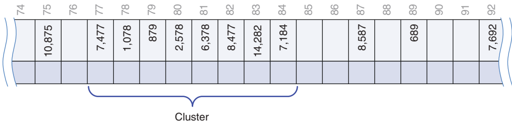
FIGURE 11-11 An example of clustering in linear addressing
