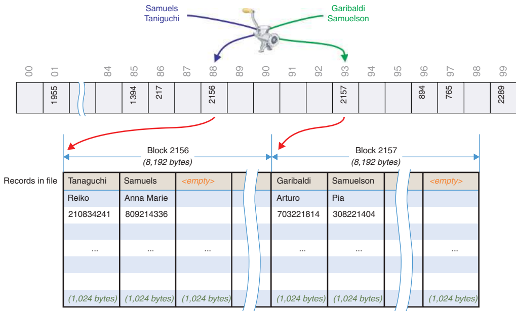
FIGURE 11-21 Hashing to external blocks
