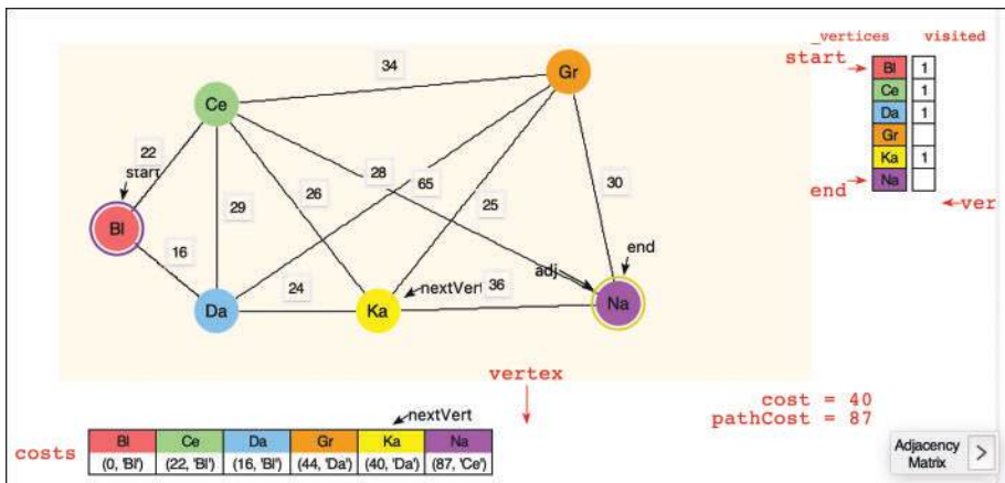
FIGURE 15-17 After selecting Ka(y) to visit in finding the shortest path to Naur
