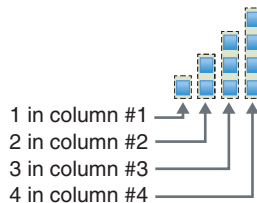
FIGURE 6-3 Triangular number as columns
