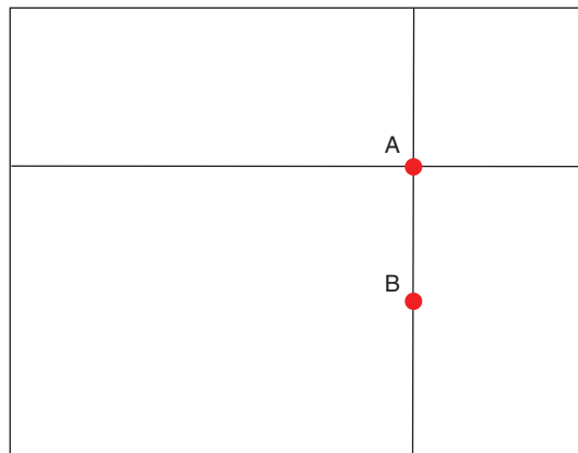
FIGURE 12-22 Quadrant ambiguity
