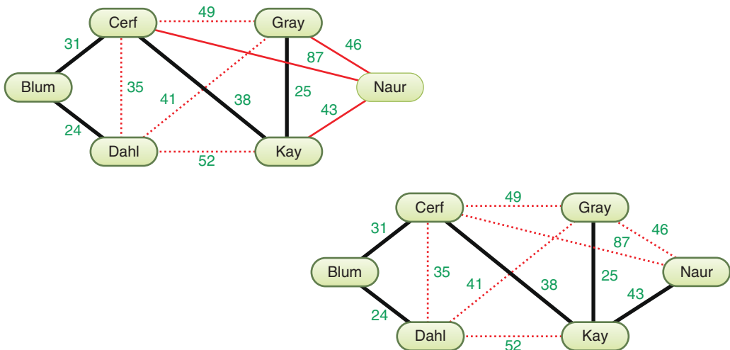
FIGURE 15-8 The final connections of the minimum spanning tree in Turala
