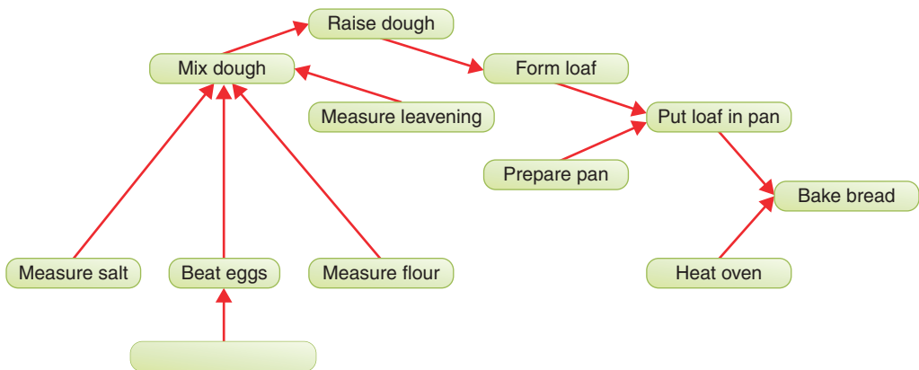
FIGURE 14-15 A dependency graph for baking bread
