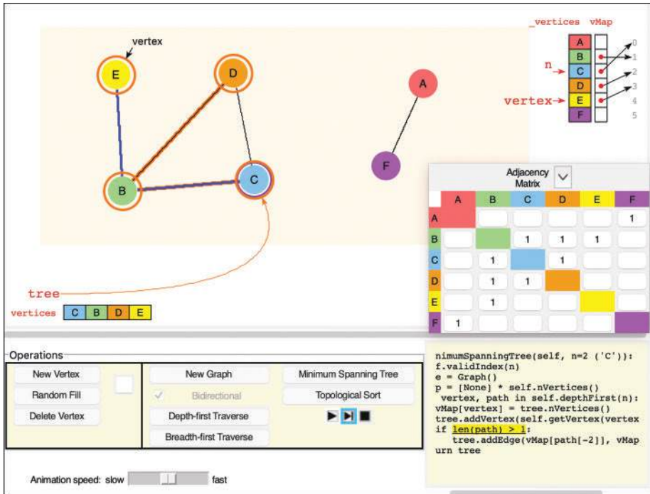
FIGURE 14-12 The Graph Visualization tool adding a path to a minimum spanning tree
