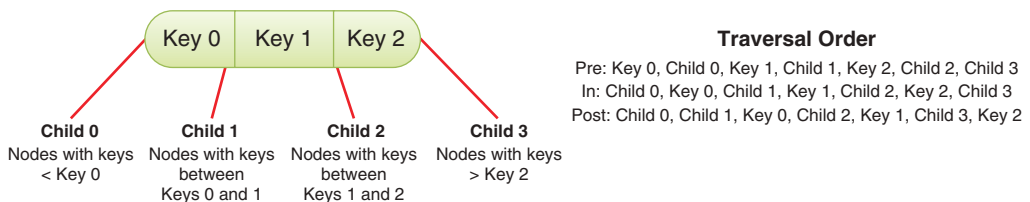
FIGURE 9-10 Traversing 2-3-4 trees
