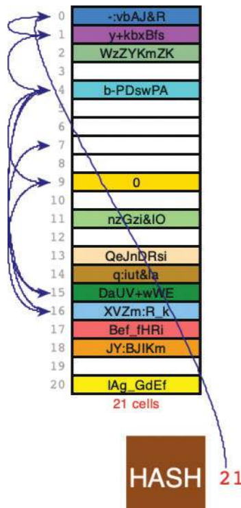
FIGURE 11-15 Inserting key 21 by quadratically probing a relatively full hash table
