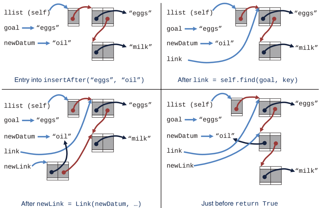
FIGURE 5-6 Inserting "oil" after "eggs" in a linked list
