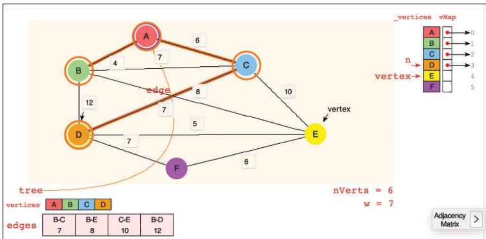
FIGURE 15-9 The Visualization tool computing a minimum spanning tree
