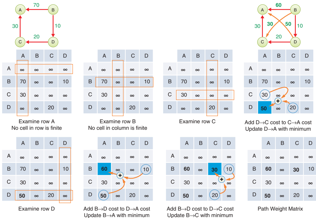
FIGURE 15-20 Steps in the Floyd-Warshall algorithm to create the path weight matrix
