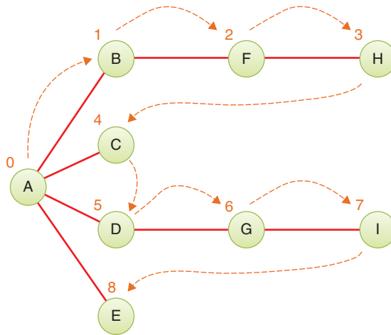
FIGURE 14-5 Depth-first traversal example
