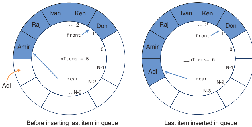
FIGURE 4-7 Inserting an item into a partially full queue
