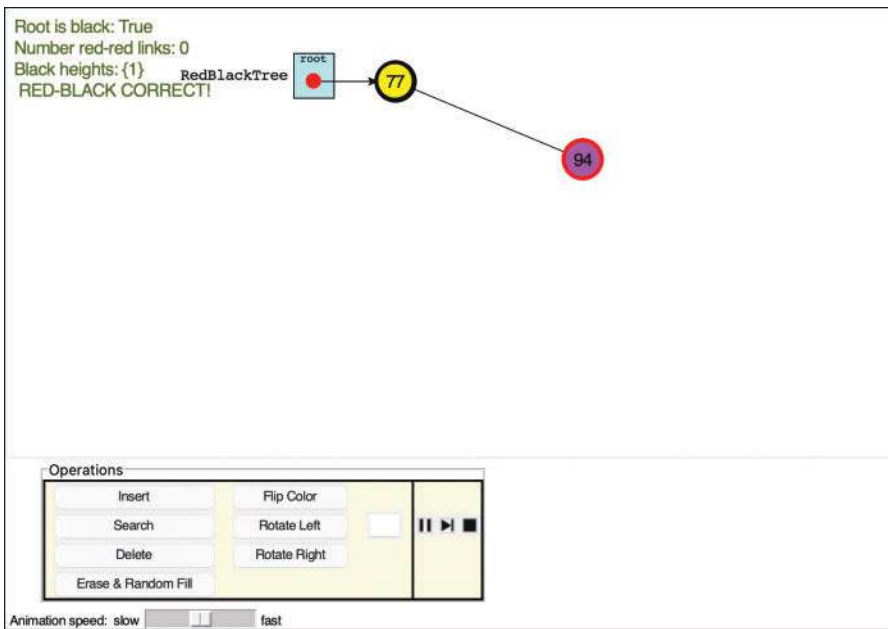
FIGURE 10-14 The RedBlackTree Visualization tool
