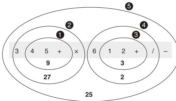
FIGURE 4-12 Visual approach to postfix evaluation of 345+×612+/-
