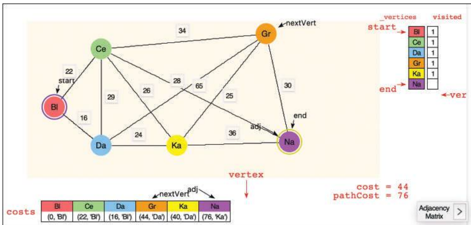
FIGURE 15-18 Visiting Gr(ay) in finding the shortest path to Naur
