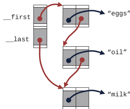
FIGURE 5-8 A double-ended list
