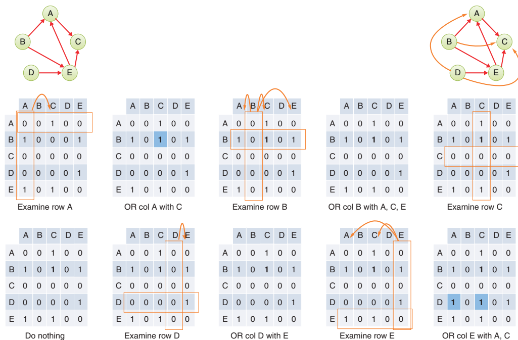
FIGURE 14-22 Steps in Warshall's algorithm
