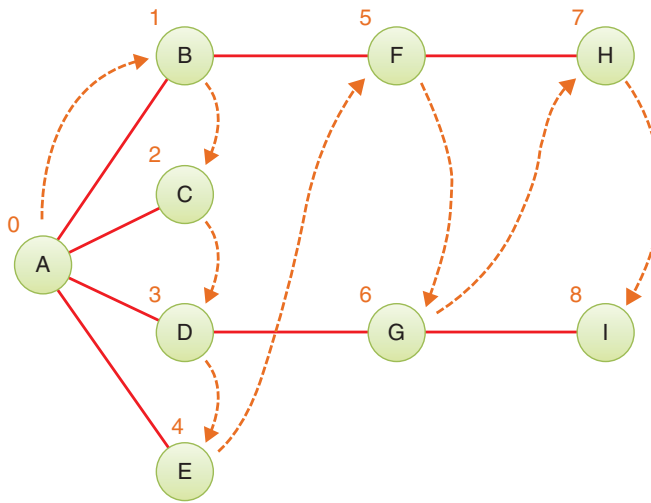
FIGURE 14-9 Breadth-first traversal example
