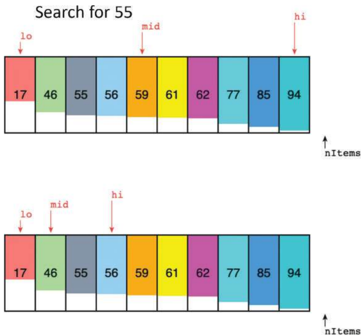
FIGURE 2-6 Initial ranges in a binary search
