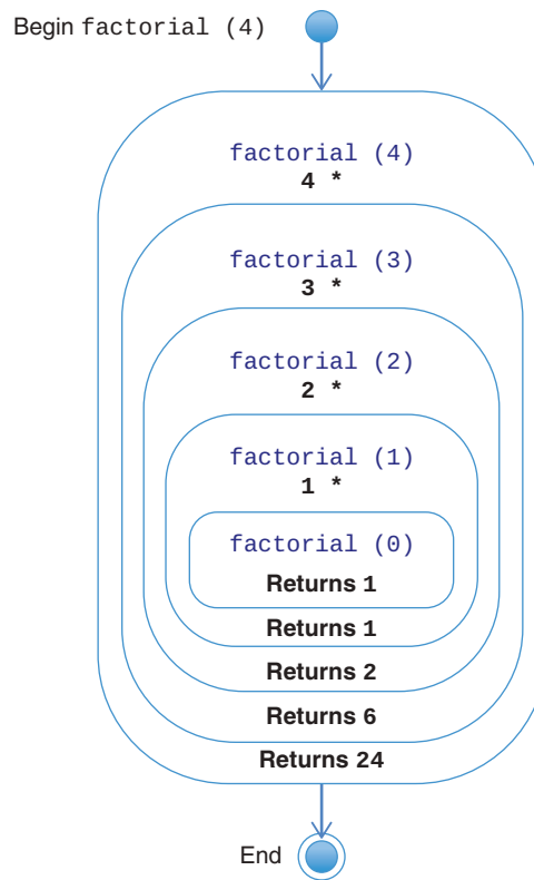
FIGURE 6-6 Execution of the recursive factorial(4) function
