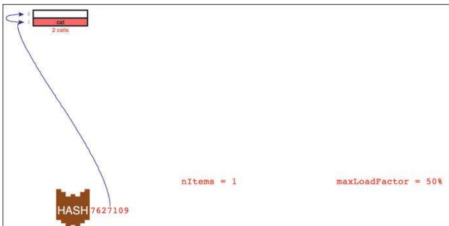
FIGURE 11-8 Probing to insert the key eat
