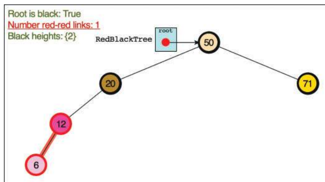
FIGURE 10-20 Parent and child are both red
