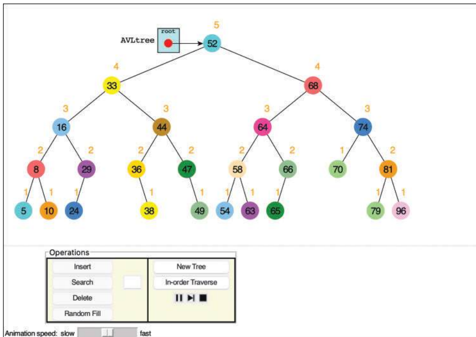
FIGURE 10-9 The AVLTree Visualization tool with a randomly filled tree
