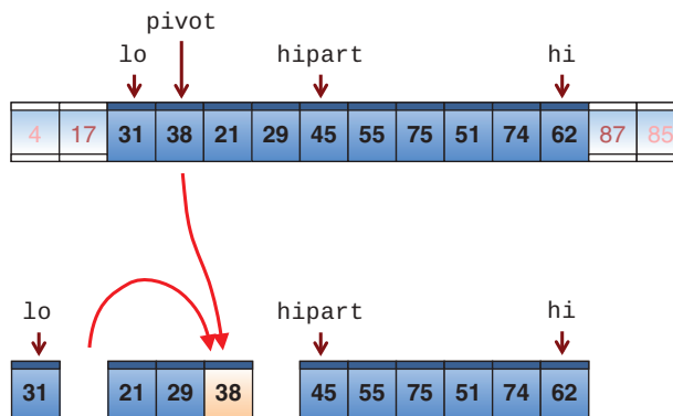
FIGURE 7-8 Moving the pivot between the subarrays
