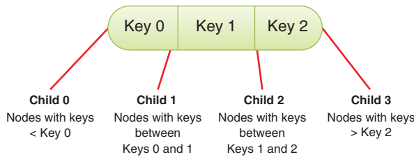
FIGURE 9-2 Keys and children
