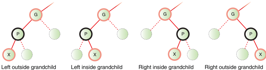
FIGURE 10-24 Handed variations of node being inserted
