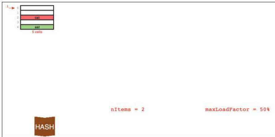
FIGURE 11-9 After inserting cat and eat in an empty hash table
