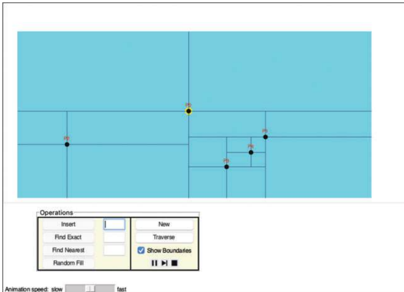
FIGURE 12-24 The QuadTree Visualization tool
