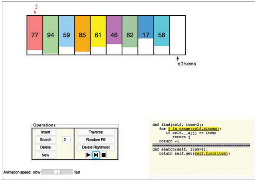
FIGURE 2-2 Starting a search for player 2
