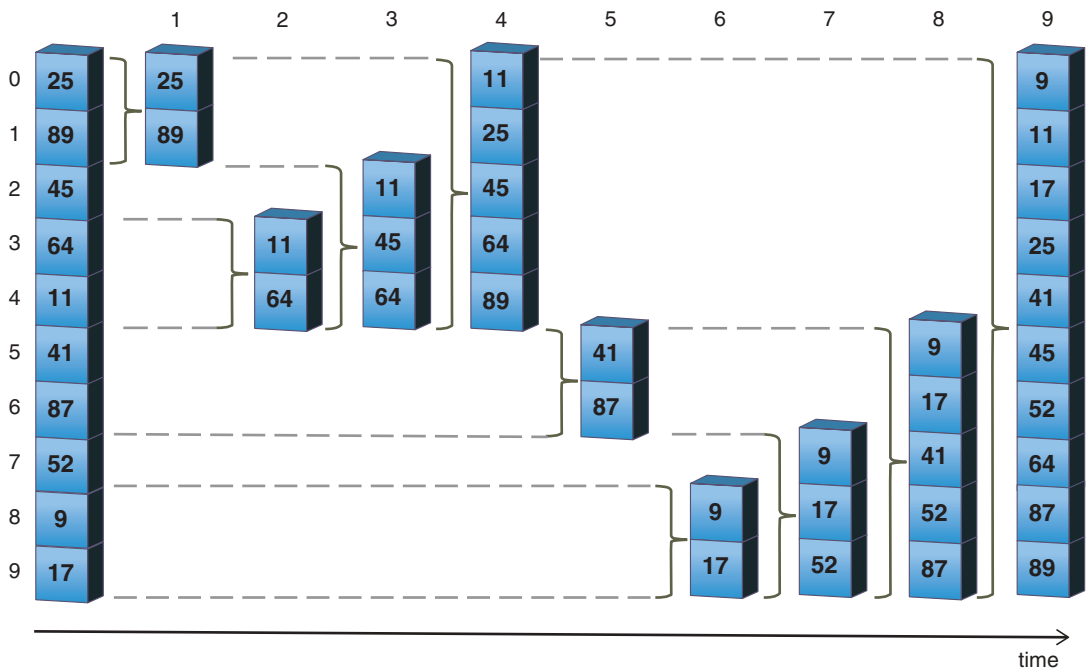
FIGURE 6-17 Mergesort when the array size not a power of 2
