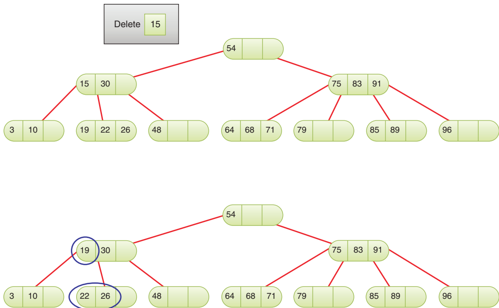
FIGURE 9-11 Deleting from an internal node by promoting the successor
