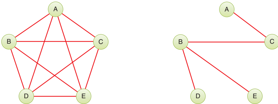
FIGURE 14-11 A fully connected graph and a minimum spanning tree
