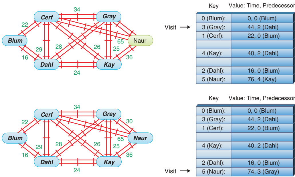
FIGURE 15-13 Following steps 4 and 5 in the shortest-path algorithm.
