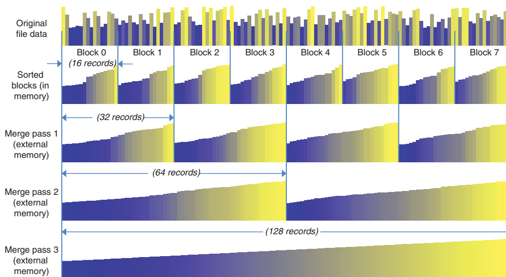
FIGURE 9-23 Mergesort on an external file
