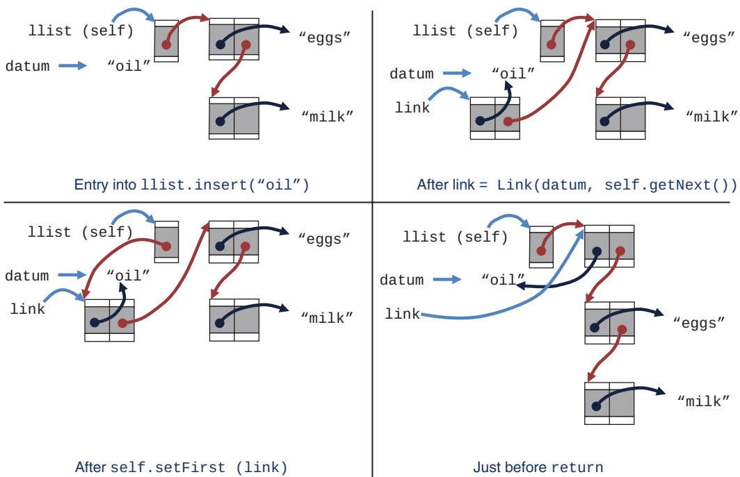
FIGURE 5-5 Execution of insert()
