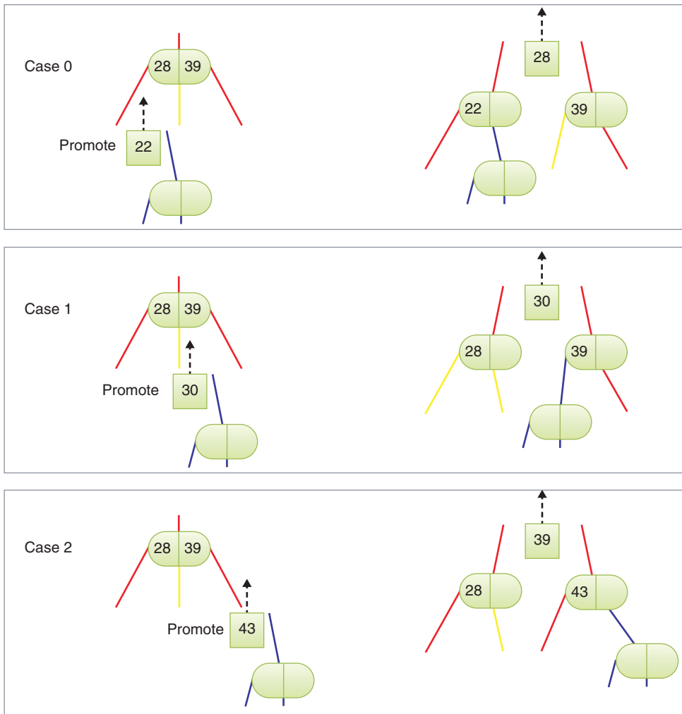
FIGURE 9-17 Splitting internal nodes
