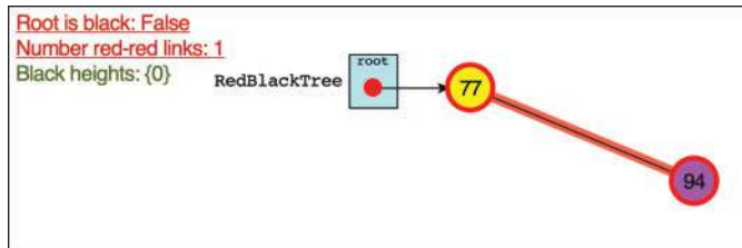
FIGURE 10-16 A tree with exactly two nodes, both red
