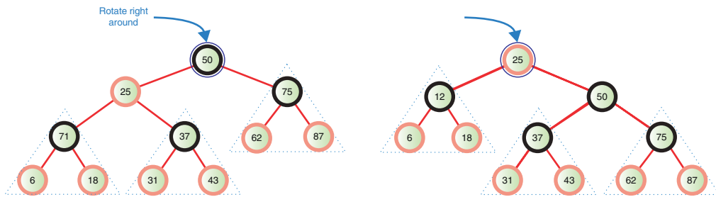
FIGURE 10-22 Subtree movement during rotation
