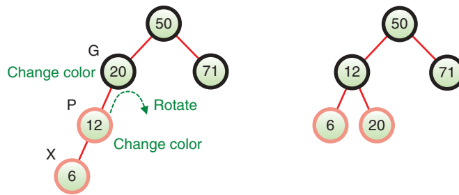
FIGURE 10-26 P is red and X is an outside grandchild
