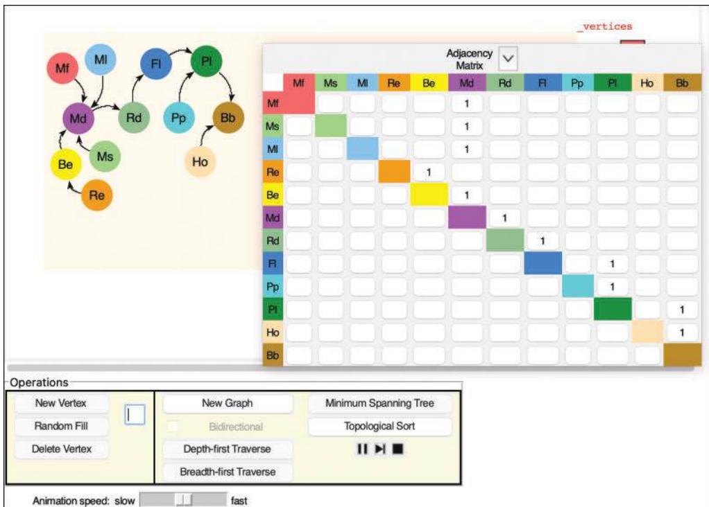
FIGURE 14-17 A directed graph in the Graph Visualization tool.
