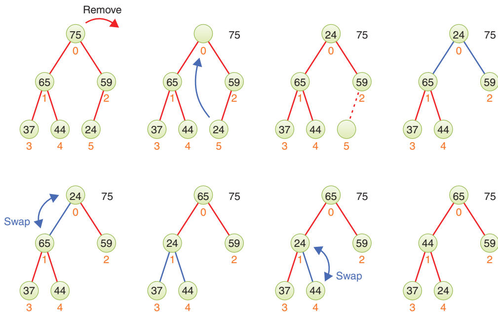
FIGURE 13-5 Replacing the root with the last item and sifting down
