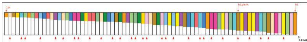
FIGURE 7-11 Running quicksort on a 77-element array choosing the rightmost as pivot
