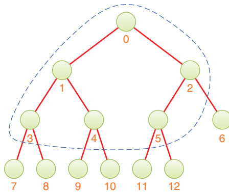
FIGURE 13-12 The _siftDown() method is applied to the internal nodes
