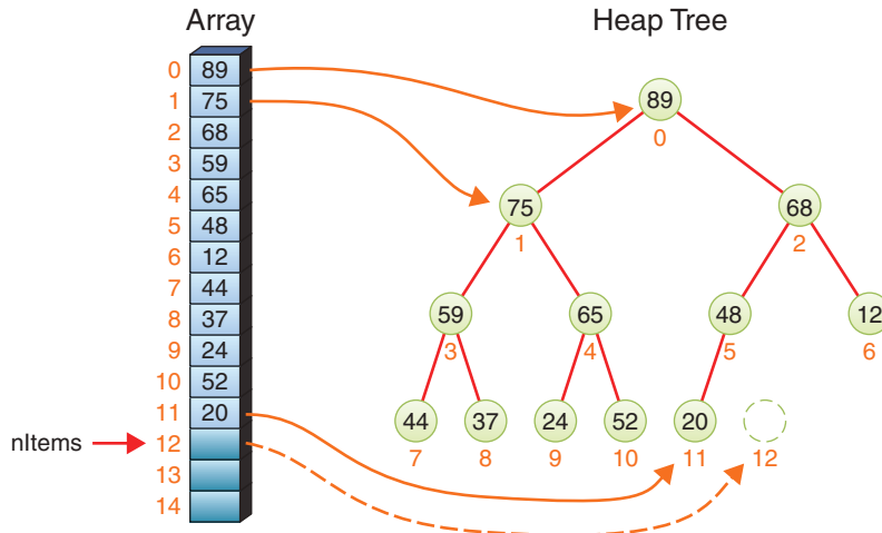
FIGURE 13-2 A heap array and its corresponding binary tree
