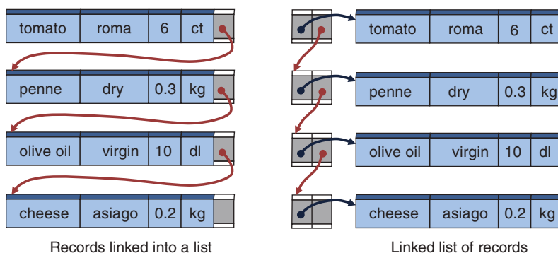
FIGURE 5-1 Different methods of representing links in a list
