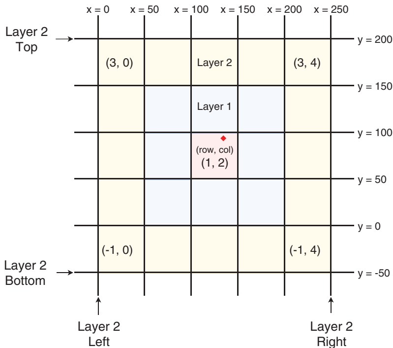
FIGURE 12-12 Determining the boundary coordinates of a layer
