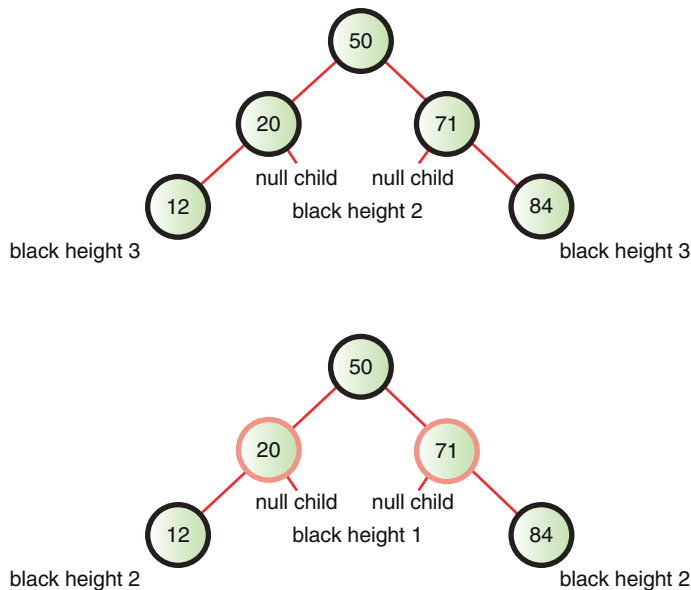
FIGURE 10-21 Paths to null children
