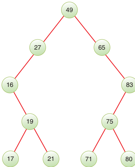
FIGURE 10-3 A symmetric binary tree
