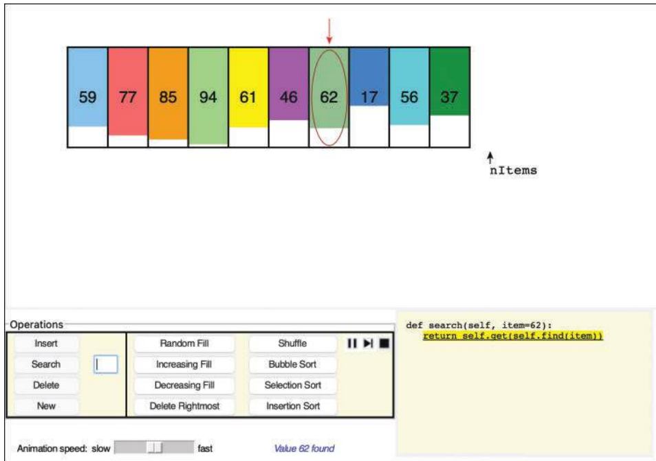
FIGURE A-4 Results of the search for key 62 in the array
