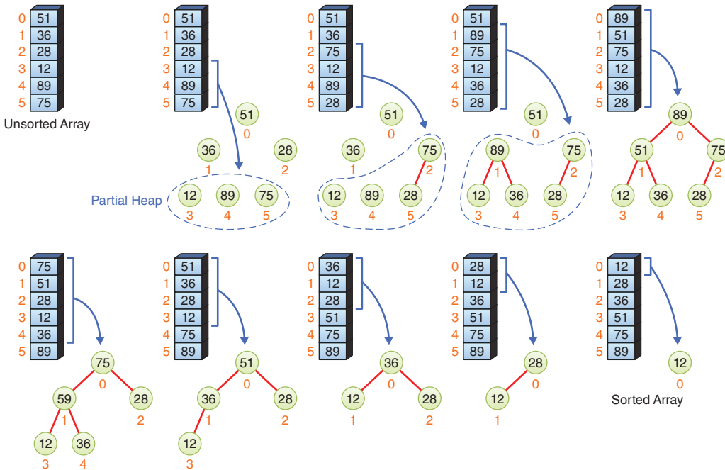
FIGURE 13-14 Heapsort in place
