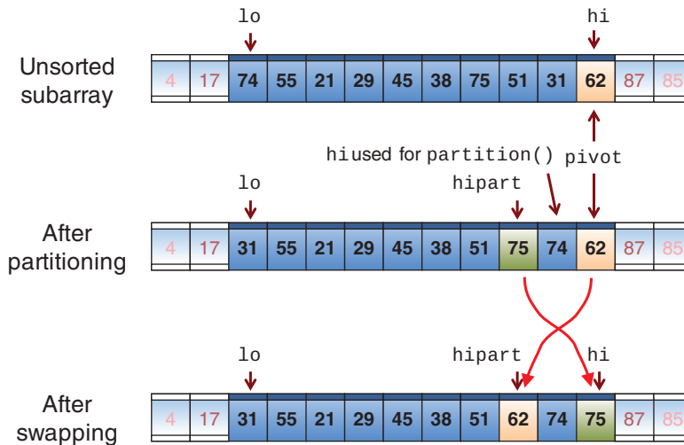
FIGURE 7-9 Swapping the pivot from the right
