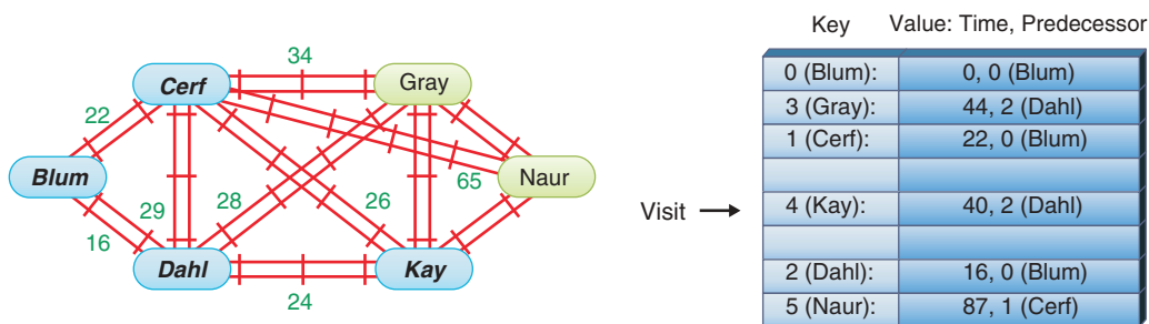
FIGURE 15-12 Following step 3 in the shortest-path algorithm.
