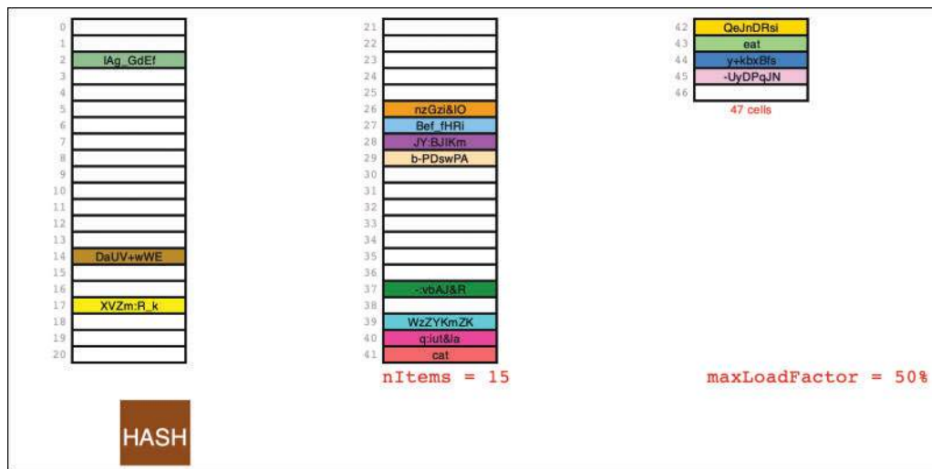
FIGURE 11-10 A hash table with 15 items
