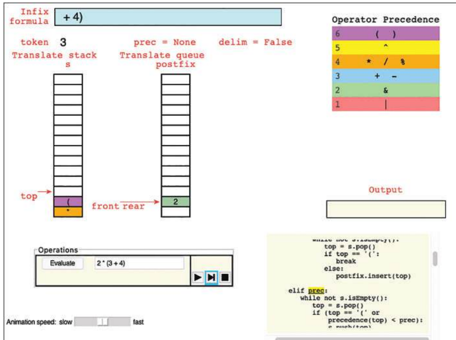
FIGURE 4-11 The InfixCalculator tool
