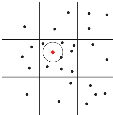
FIGURE 12-9 Finding the nearest match in a grid
