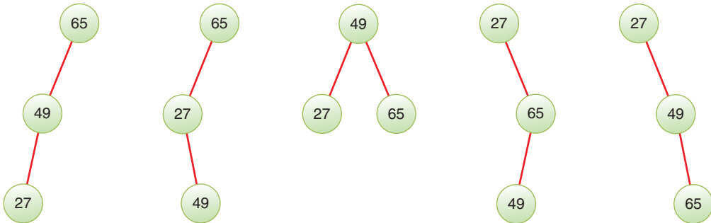
FIGURE 10-6 The possible shapes for 3-node binary search trees
