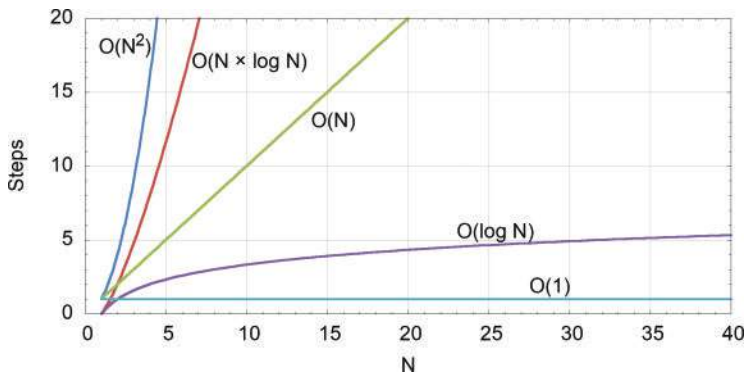
FIGURE 2-8 Graph of Big O times
