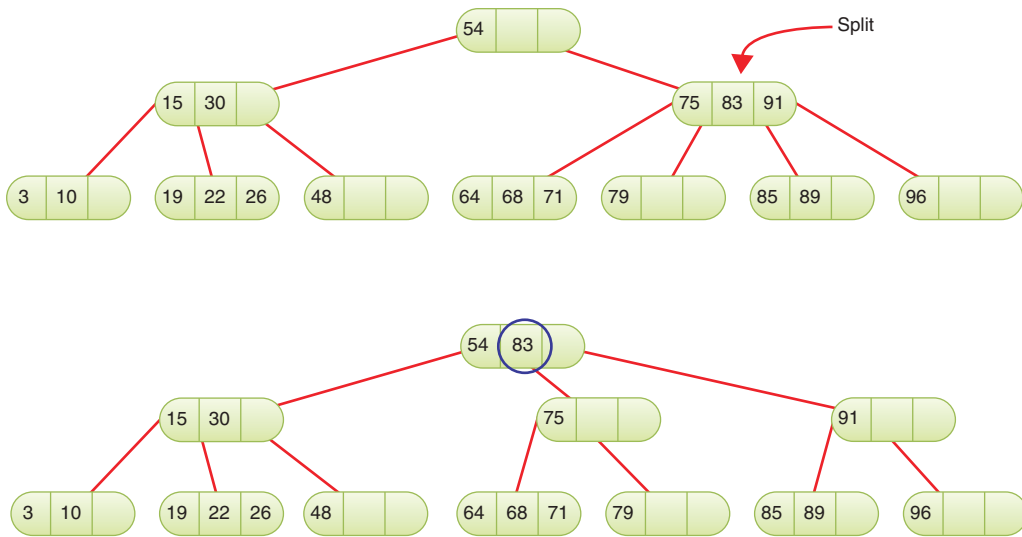
FIGURE 9-4 Splitting a nonroot node
