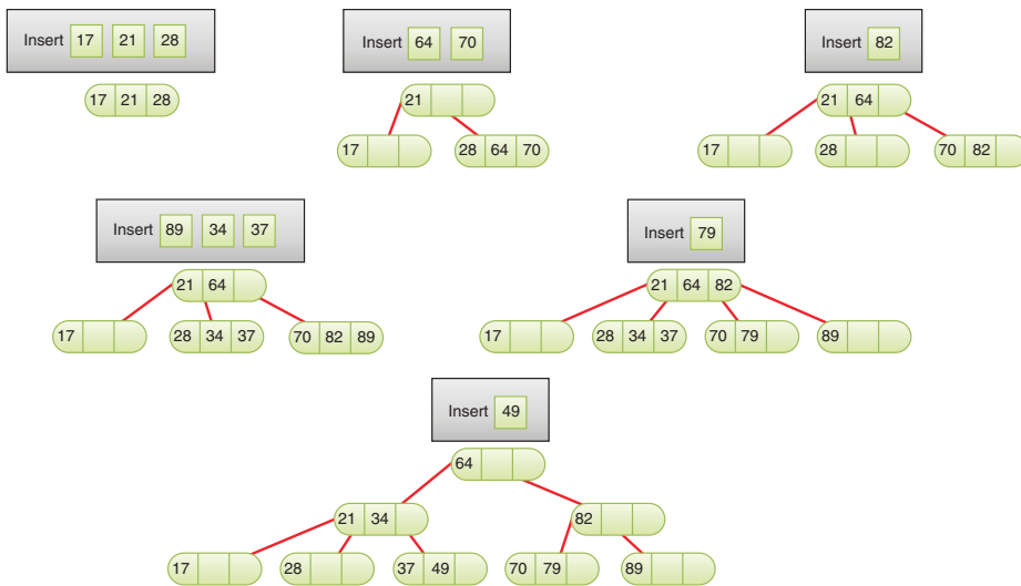
FIGURE 9-6 Insertions into a 2-3-4 tree
