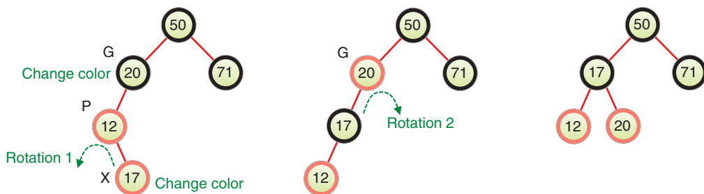
FIGURE 10-27 P is red and X is an inside grandchild
