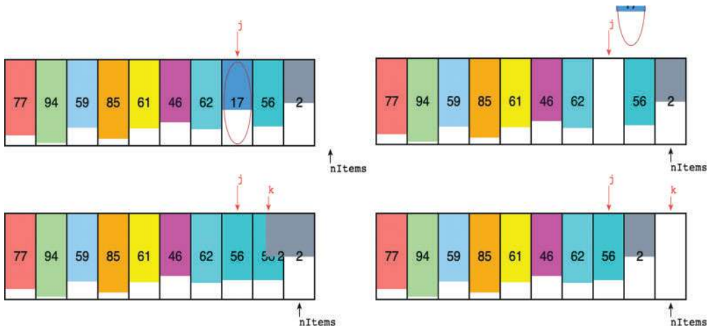
FIGURE 2-3 Deleting an item
