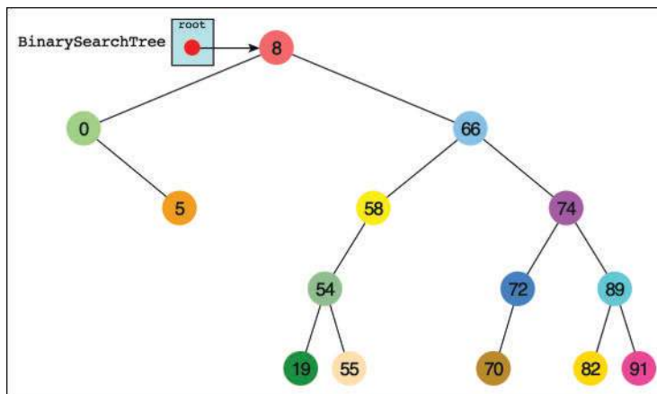
FIGURE 10-2 A partially unbalanced tree
