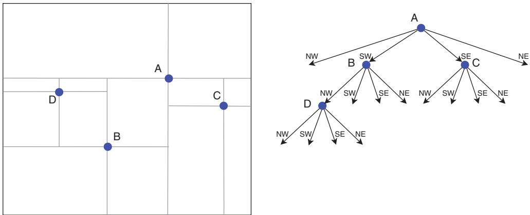
FIGURE 12-21 Inserting point D
