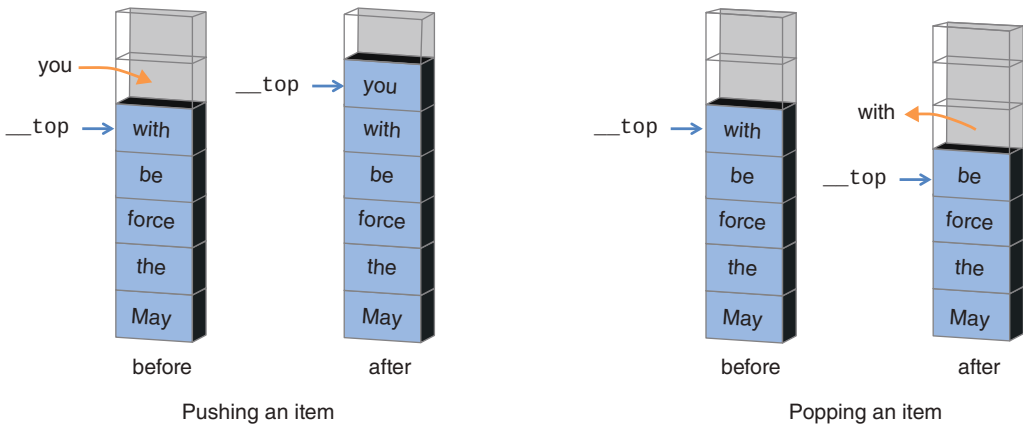
FIGURE 4-3 Operation of the Stack class push() and pop() methods
