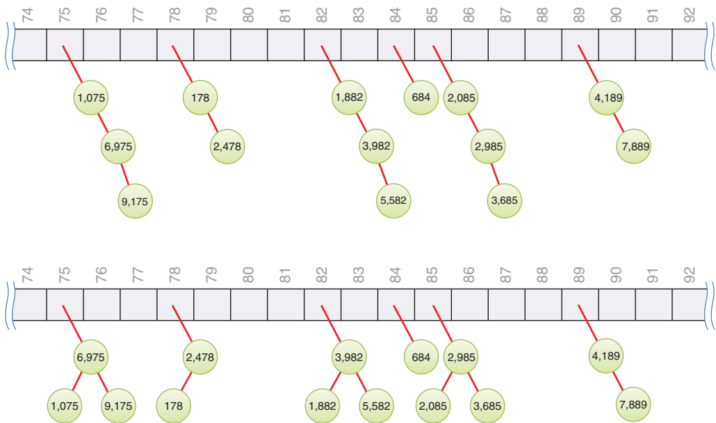
FIGURE 11-17 Examples of separate chaining
