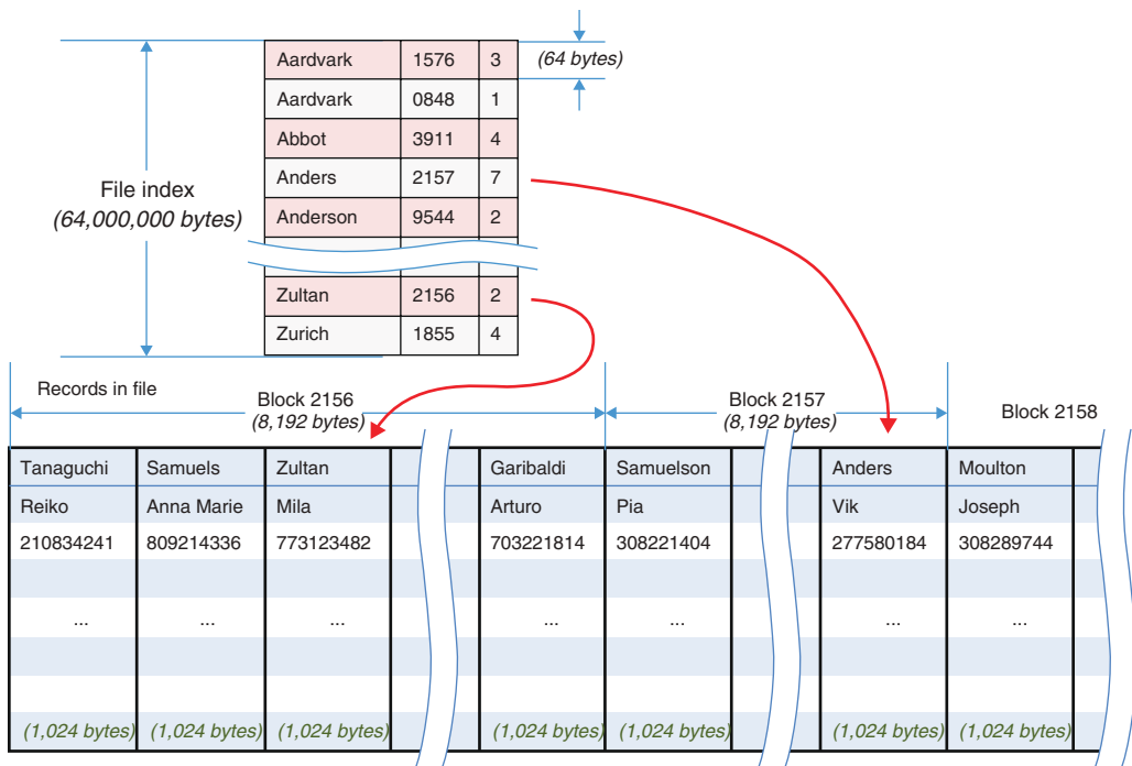
FIGURE 9-22 A file index example
