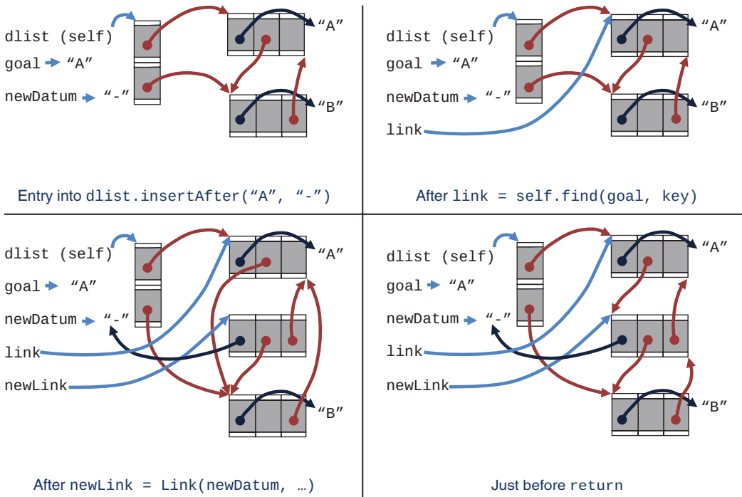
FIGURE 5-13 Insertion in the middle of a doubly linked list
