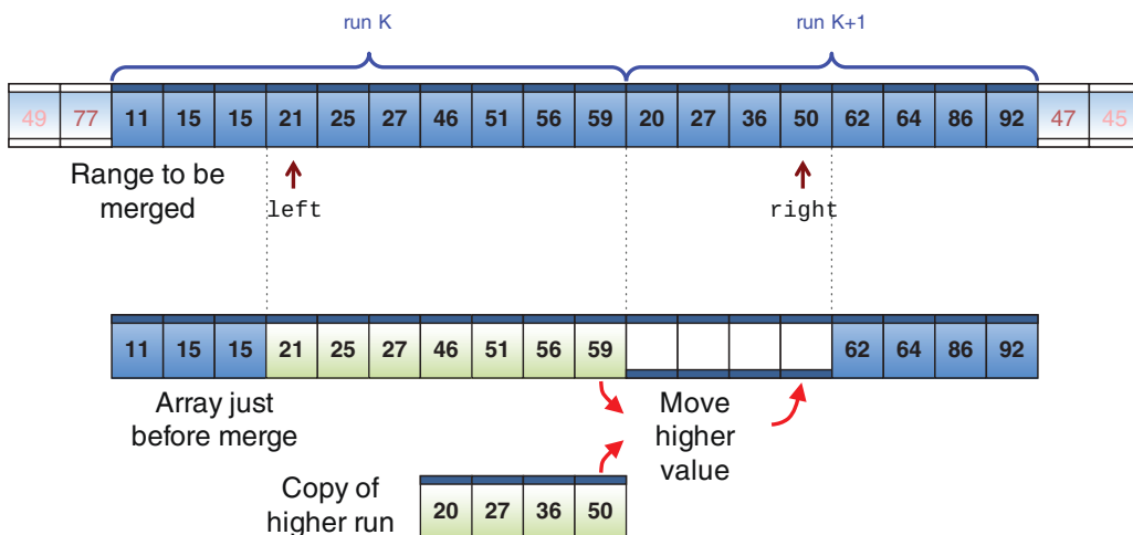
FIGURE 7-18 Merging adjacent runs in Timsort
