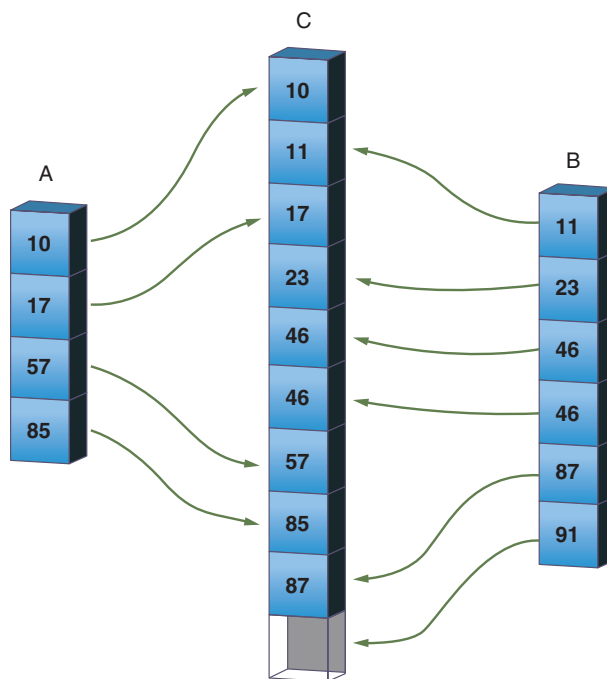
FIGURE 6-15 Merging two arrays
