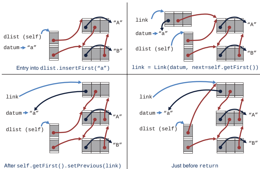
FIGURE 5-11 Insertion at the beginning of a doubly linked list
