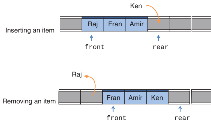
FIGURE 4-4 Queue operations in a linear array
