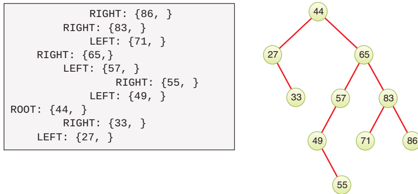
FIGURE 8-25 Tree printed with indentation for node depth
