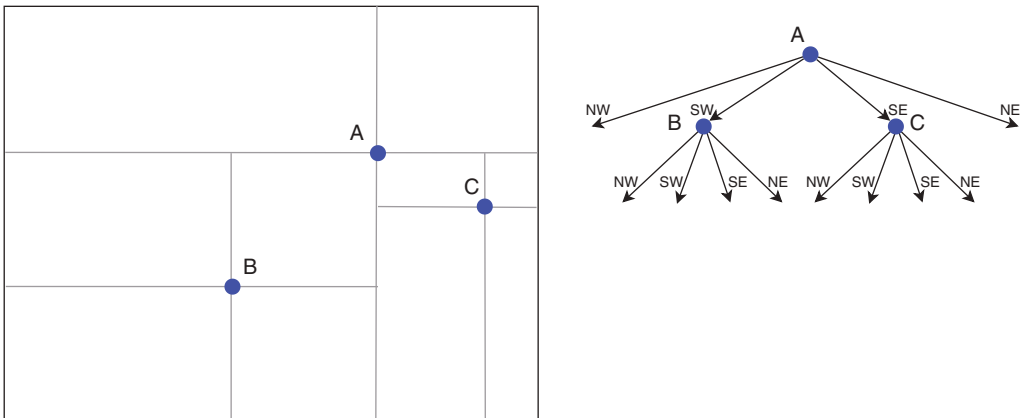
FIGURE 12-20 Inserting point C
