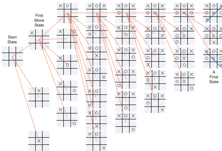
FIGURE 14-8 Tic-tac-toe board states as a graph
