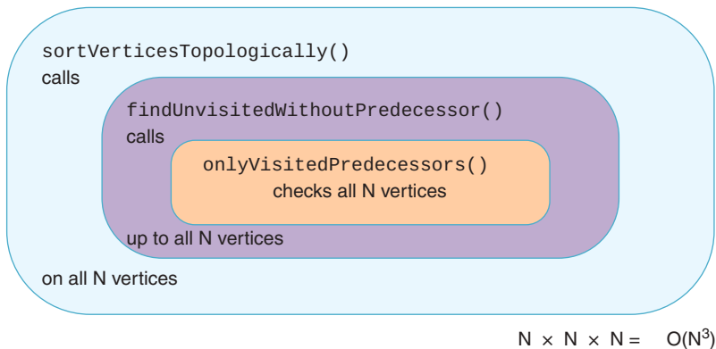
FIGURE 14-19 Complexity of the basic topological sort algorithm
