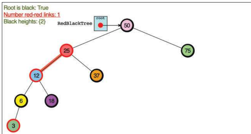
FIGURE 10-29 Correcting a red-red outside grandchild in the Visualization tool
