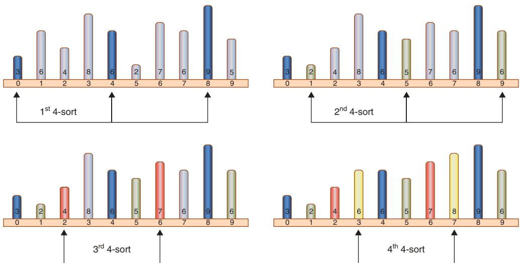
FIGURE 7-2 A complete 4-sort
