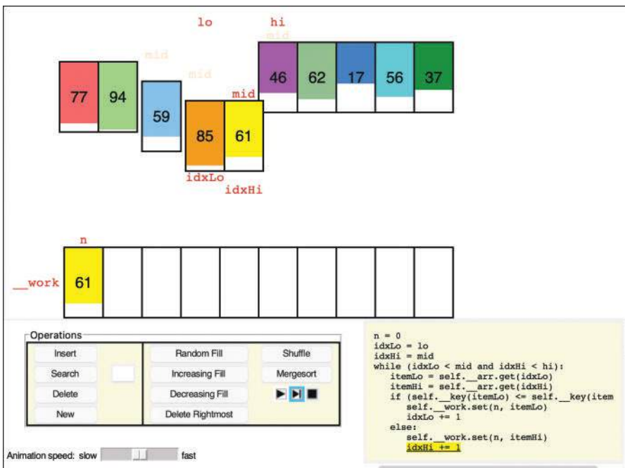
FIGURE 6-18 The Mergesort Visualization tool
