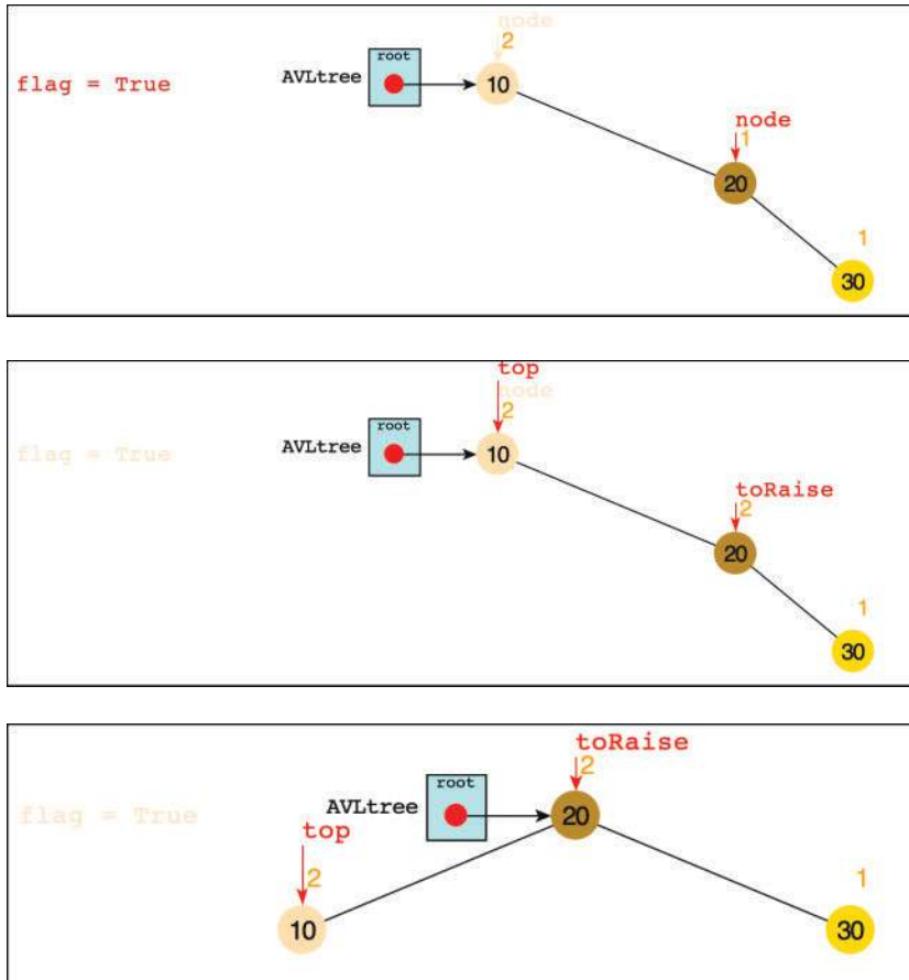
FIGURE 10-11 Steps in the insertion of node 30 into the AVL tree
