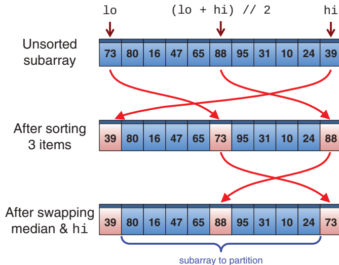
FIGURE 7-14 Sorting the left, center, and right elements
