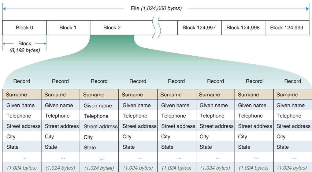
FIGURE 9-18 Blocks and records in a file
