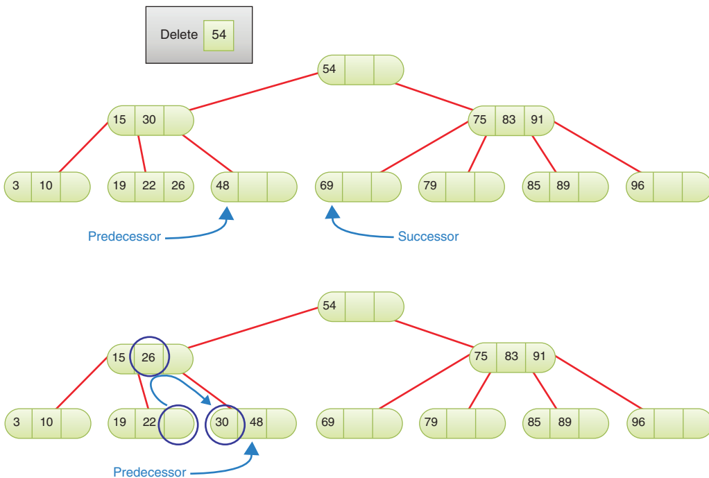
FIGURE 9-12 Deleting an item by rotating items into the predecessor node
