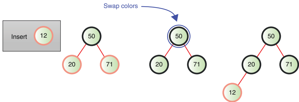
FIGURE 10-19 Inserting a node with a color swap
