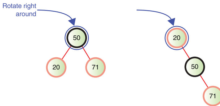
FIGURE 10-18 The right rotation operation
