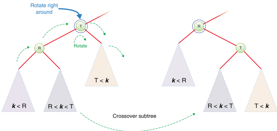
FIGURE 10-12 Right rotation and the crossover subtree
