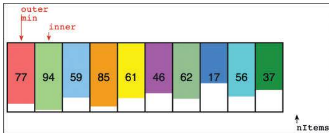
FIGURE 3-7 The start of a selection sort in the SimpleSorting Visualization tool
