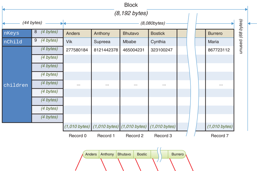
FIGURE 9-20 A node in a B-tree of order 9 with its block structure
