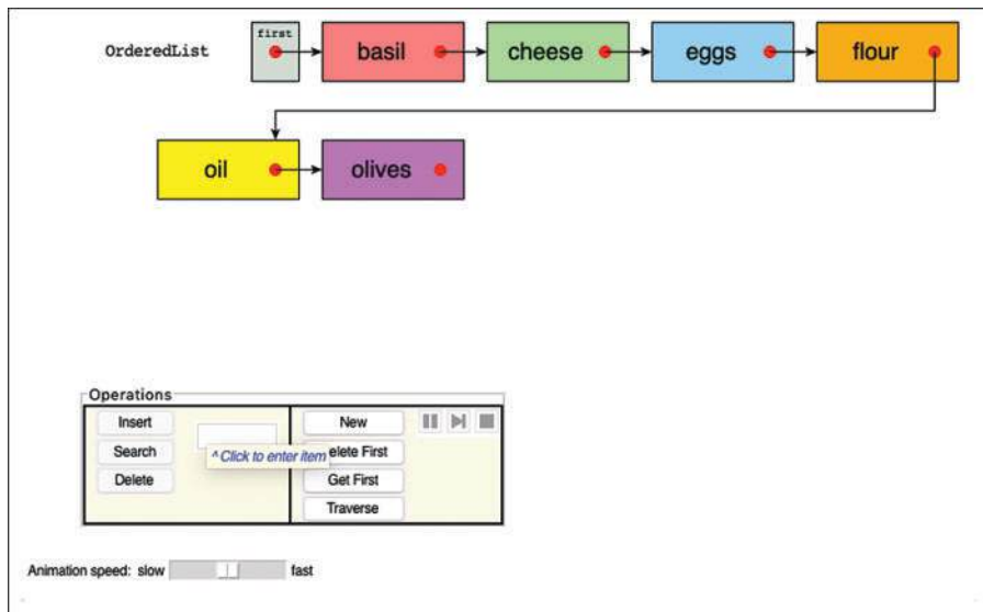
FIGURE 5-9 The OrderedList Visualization tool
