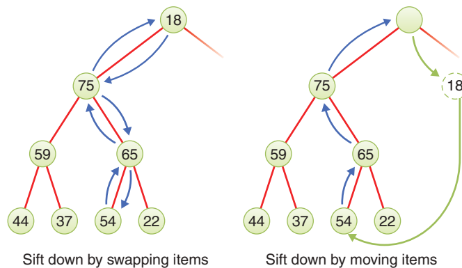
FIGURE 13-6 Sifting down with swaps versus with moves
