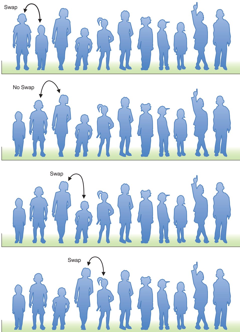
FIGURE 3-3 Bubble sort: swaps made during the first pass
