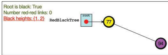
FIGURE 10-15 A tree with exactly two nodes, both black
