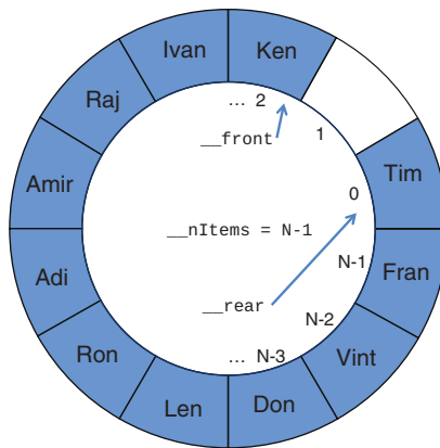
Items in queue wrapping around
