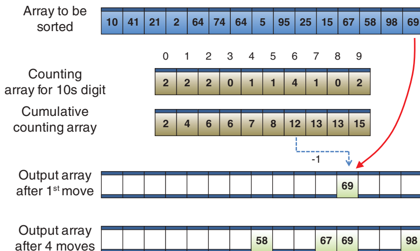
FIGURE 7-16 Applying the counting sort on the 10s digit
