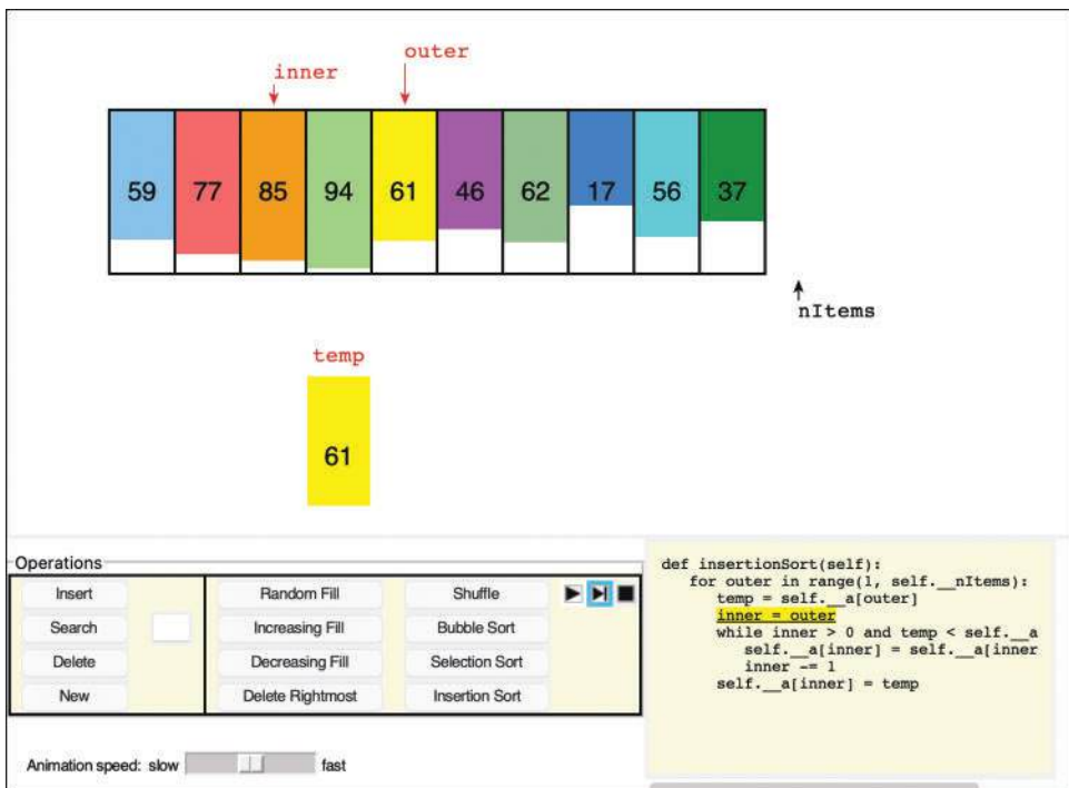
FIGURE A-3 The code box in the lower right
