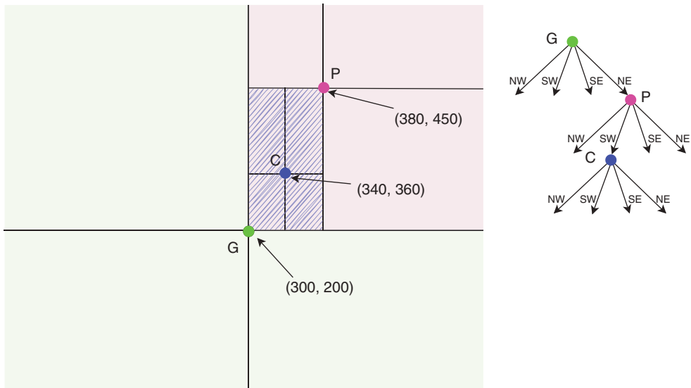
FIGURE 12-26 The intersection of ancestor quadrants forms a child's quadrant
