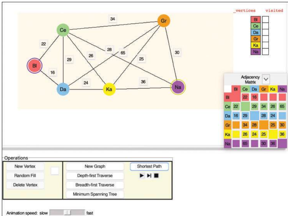
FIGURE 15-14 The railroad scenario in WeightedGraph Visualization tool
