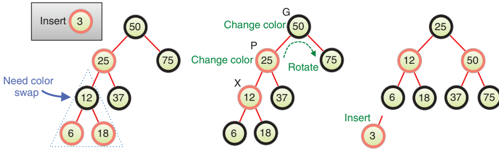
FIGURE 10-28 Correcting a red-red outside grandchild on the way down
