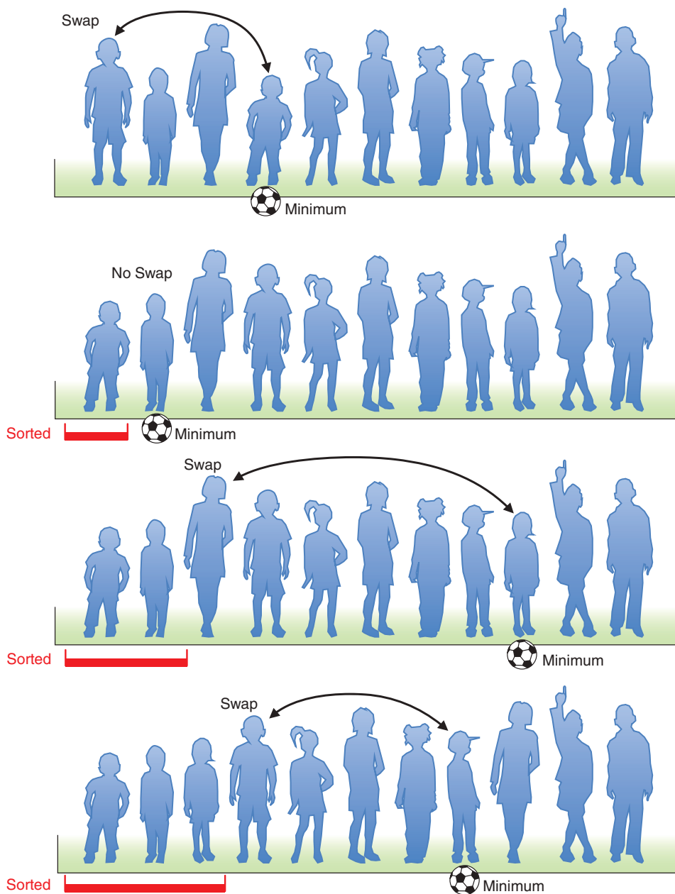
FIGURE 3-6 Selection sort on football players
