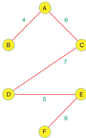
FIGURE 15-3 The minimum spanning tree of the previous graph
