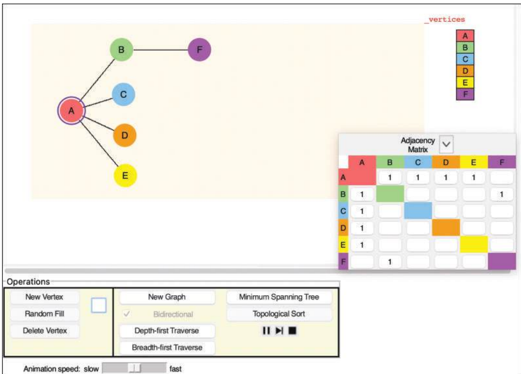
FIGURE 14-6 The Graph Visualization tool
