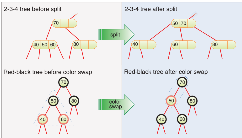
FIGURE 10-34 A 4-node split and color swap
