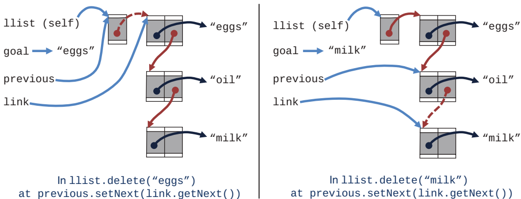
FIGURE 5-7 Two examples of deleting a Link from a LinkedList
