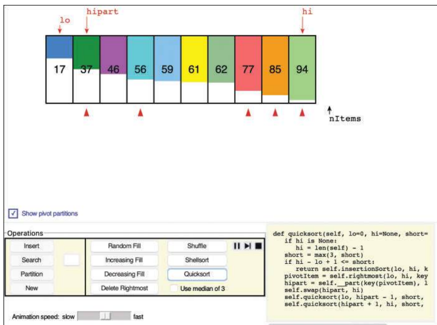
FIGURE 7-10 The result of quicksort in the AdvancedSorting Visualization tool
