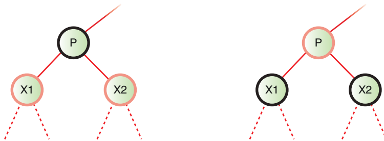
FIGURE 10-23 Color swap
