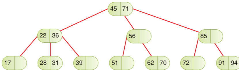
FIGURE 9-15 A 2-3 tree
