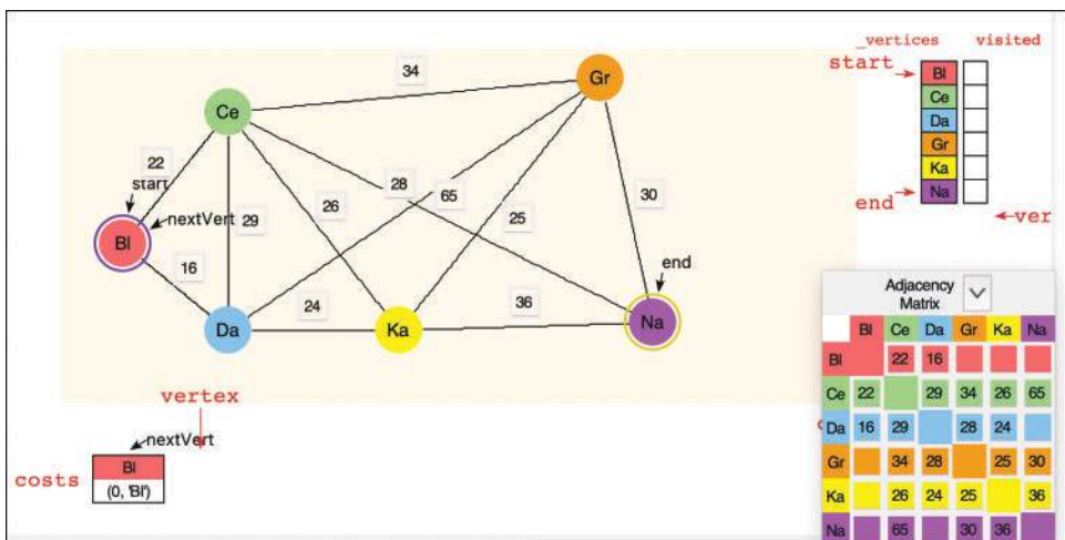
FIGURE 15-15 The first entry in costs for the shortest path to Naur
