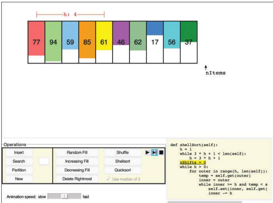
FIGURE 7-3 The AdvancedSorting Visualization tool
