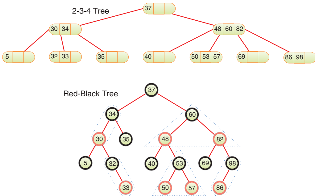
FIGURE 10-33 A 2-3-4 tree and its red-black equivalent
