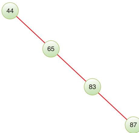
FIGURE 10-1 Unbalanced tree resulting from items inserted in ascending order
