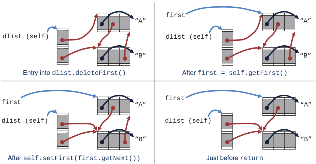
FIGURE 5-12 Deleting the first item of a doubly linked list
