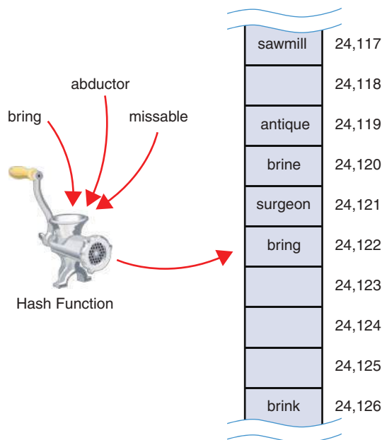
FIGURE 11-4 A collision
