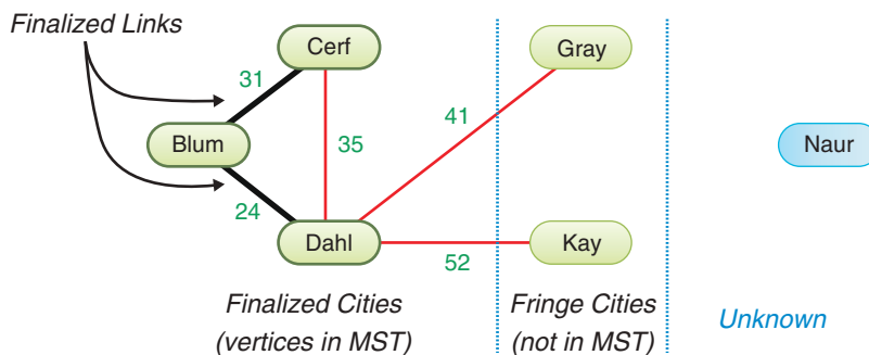
FIGURE 15-6 Partway through the minimum spanning tree algorithm
