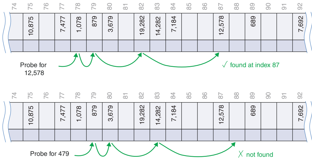
FIGURE 11-13 Quadratic probes
