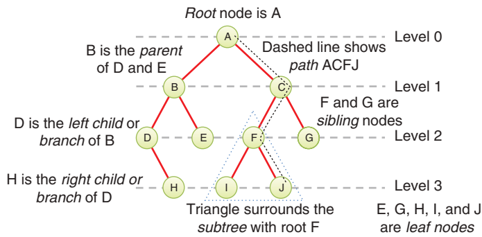
FIGURE 8-2 Tree terms
