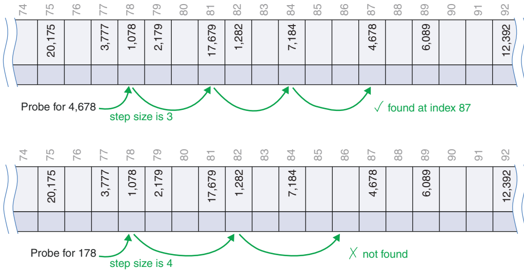
FIGURE 11-16 Double hashing
