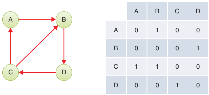
FIGURE 14-18 Directed graph with cycles.
