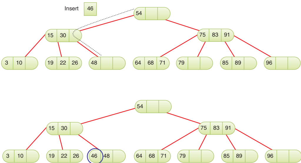
FIGURE 9-3 Insertion with no splits
