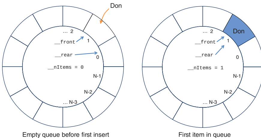
FIGURE 4-5 Operation of the Queue.insert() method on an empty queue
