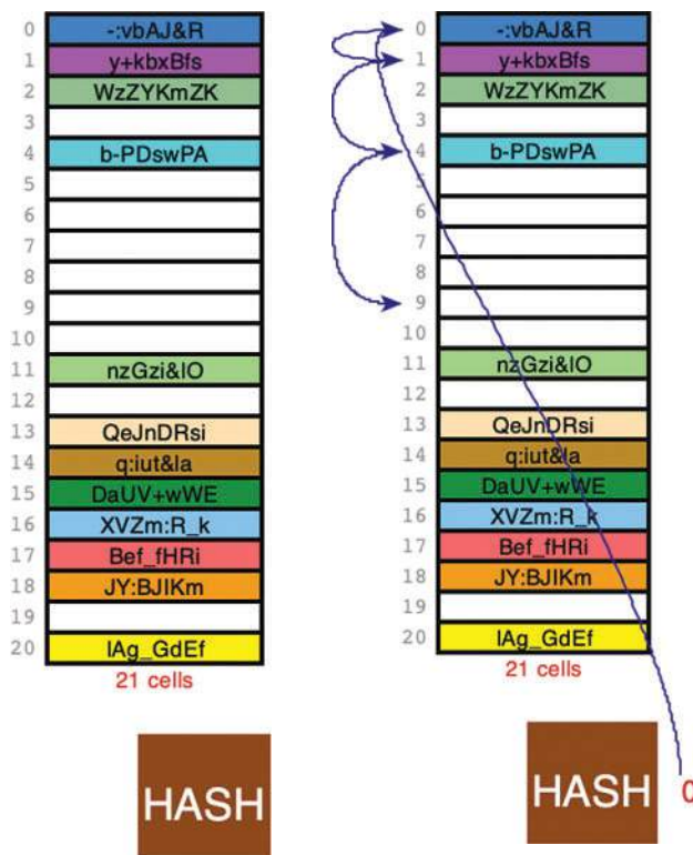
FIGURE 11-14 Quadratic probing in the HashTableOpenAddressing Visualization tool
