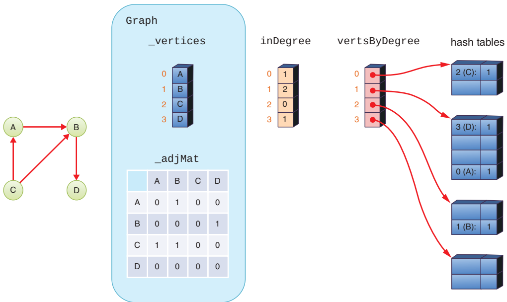
FIGURE 14-20 Structures used for topological sort
