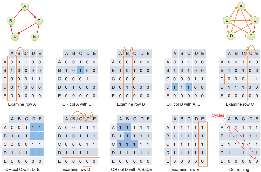
FIGURE 14-24 Marshall's algorithm applied to a graph with a cycle
