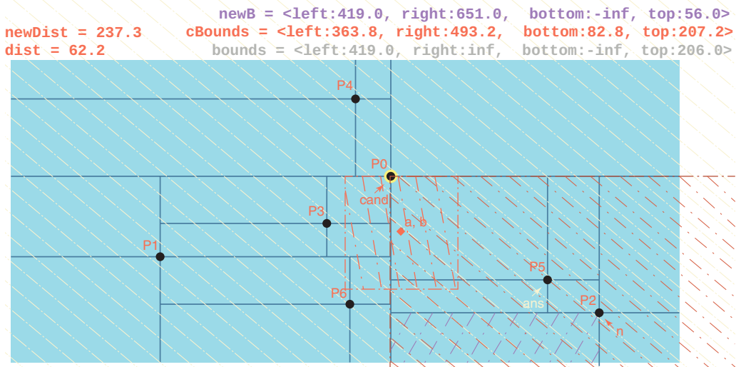
FIGURE 12-29 Eliminating quadrants during find nearest search
