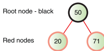
FIGURE 10-17 A balanced tree
