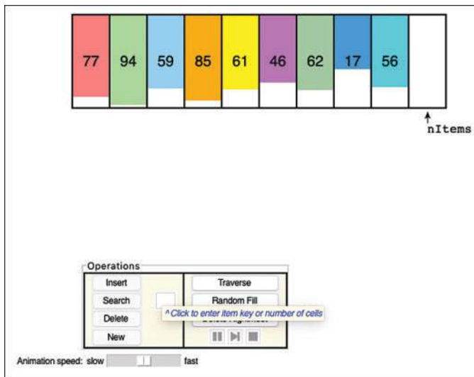
FIGURE A-2 Drawing area at the top and a set of controls on the bottom
