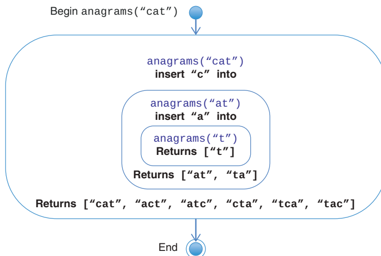
FIGURE 6-7 Anagramming a word
