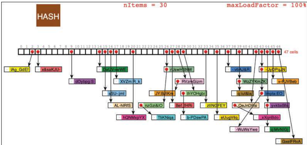
FIGURE 11-19 A separate chaining hash table with 30 random items
