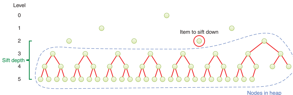
FIGURE 13-16 Sifting down during heapify
