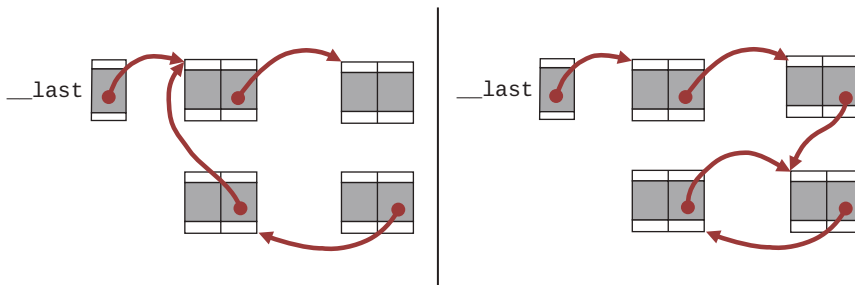
FIGURE 5-15 Broken circular lists (without data)
