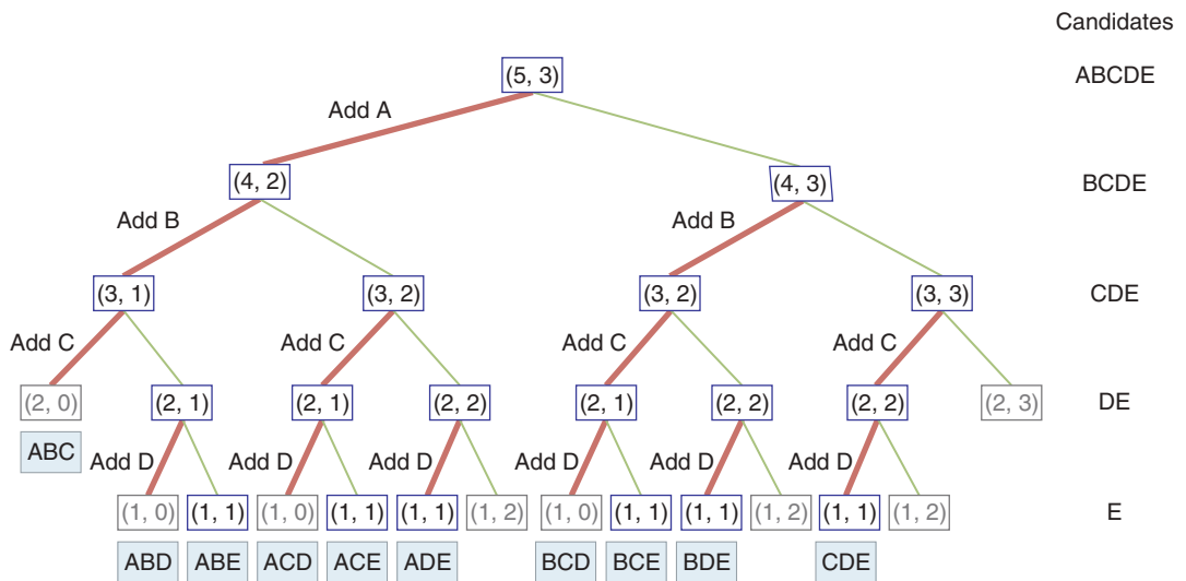
FIGURE 6-19 Picking a team of 3 from a group of 5
