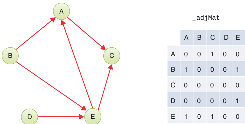
FIGURE 14-21 A five-vertex directed graph and its adjacency matrix
