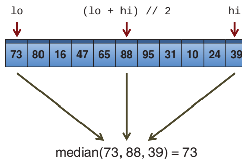
FIGURE 7-13 The median of three
