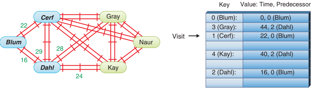
FIGURE 15-11 Following step 2 in the shortest-path algorithm.
