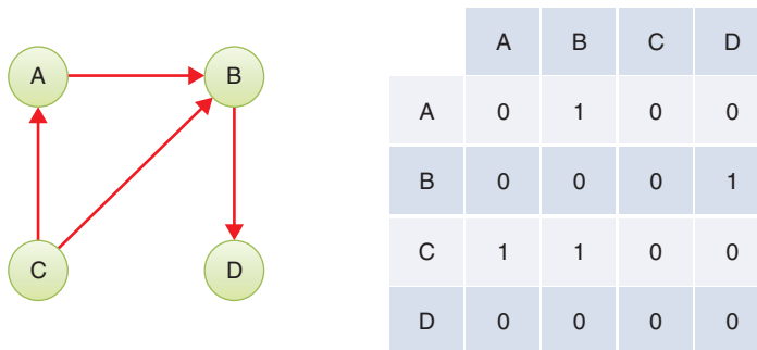
FIGURE 14-16 A small directed graph and its adjacency matrix
