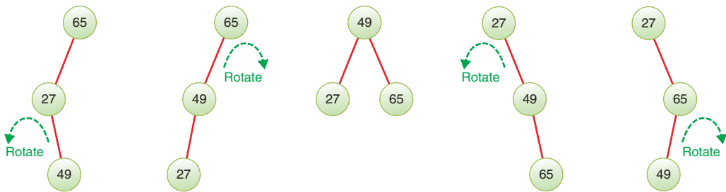
FIGURE 10-8 Rotations on 3-node binary search trees
