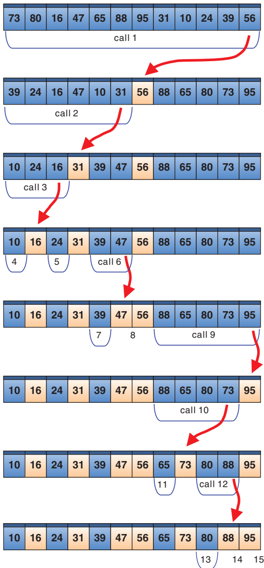
FIGURE 7-12 The qsort process
