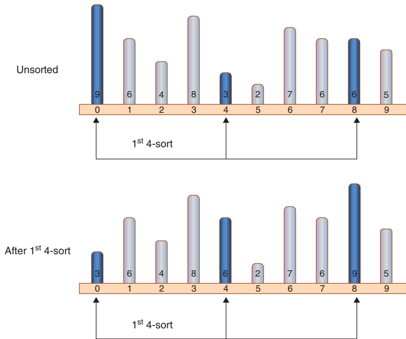
FIGURE 7-1 4-sorting at 0, 4, and 8
