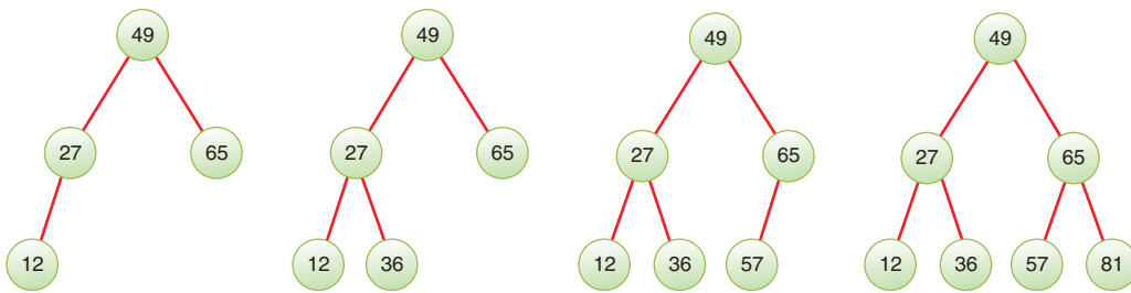
FIGURE 10-7 Balanced 4-, 5-, 6-, and 7-node binary search trees
