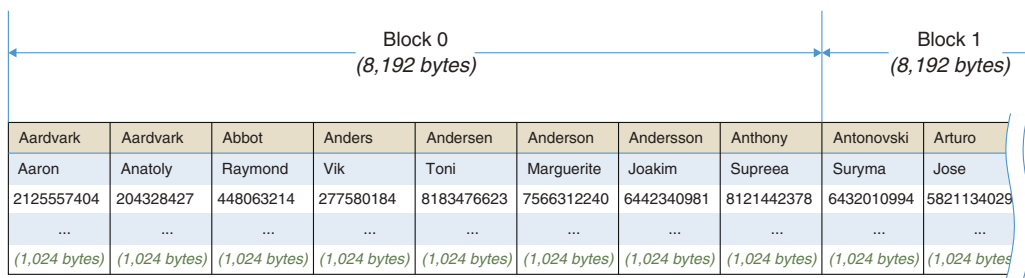
FIGURE 9-19 Sequential ordering of records
