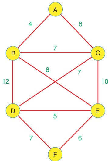
FIGURE 15-1 A weighted graph
