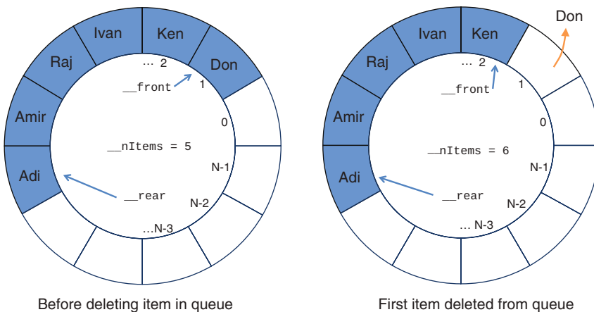
FIGURE 4-8 Deleting an item from the queue
