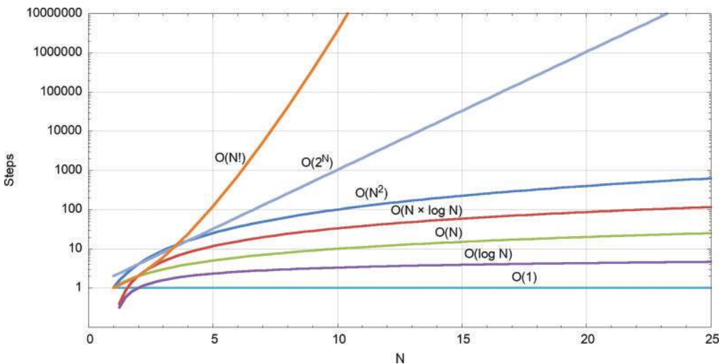
FIGURE 15-22 Exponential growth
