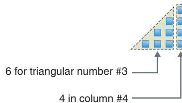
FIGURE 6-4 Triangular number as column plus triangle
