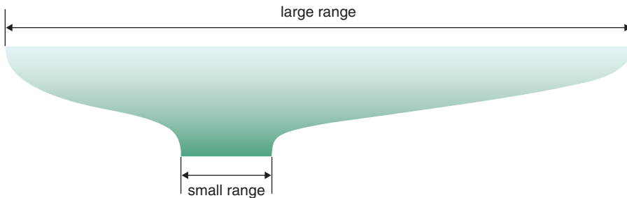
FIGURE 11-3 Range conversion using modulo
