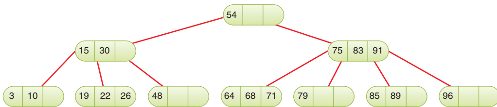
FIGURE 9-1 A 2-3-4 tree
