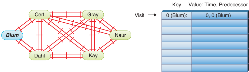
FIGURE 15-10 Train travel in Turala
