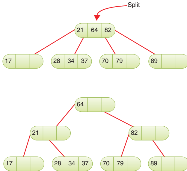
FIGURE 9-5 Splitting the root
