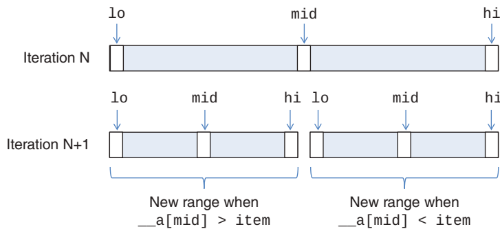
FIGURE 2-7 Dividing the range in a binary search
