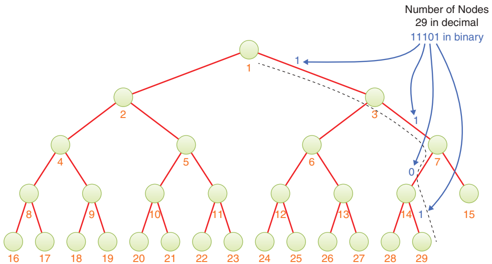
FIGURE 13-10 Finding the path to the last node in a 29-node tree.
