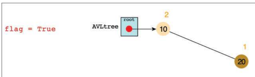
FIGURE 10-10 The first two items inserted in an AVL tree
