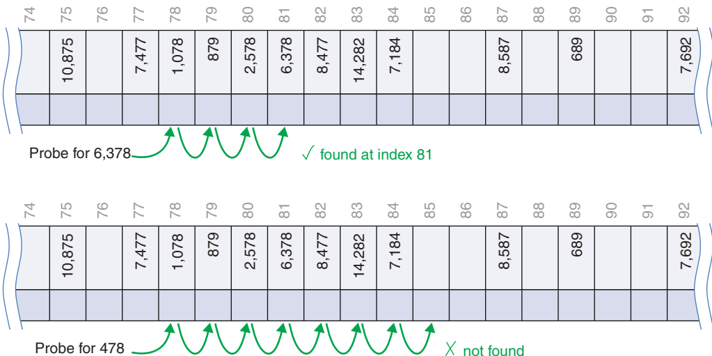
FIGURE 11-12 Linear probes in clusters Humble Bundle Pearson Python Bundle – © Pearson. Do Not Distribute.
