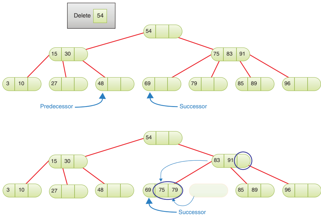
FIGURE 9-13 Deleting an item by fusing items into the successor node
