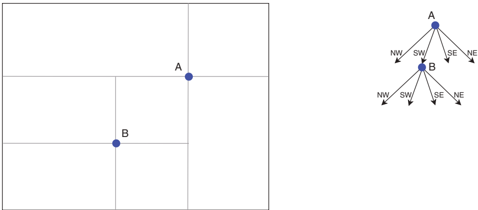
FIGURE 12-19 Inserting point B
