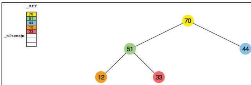
FIGURE 13-8 A small heap in the Heap Visualization tool
