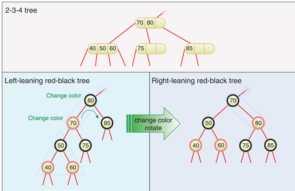
FIGURE 10-35 3-node transformation and equivalent rotation
