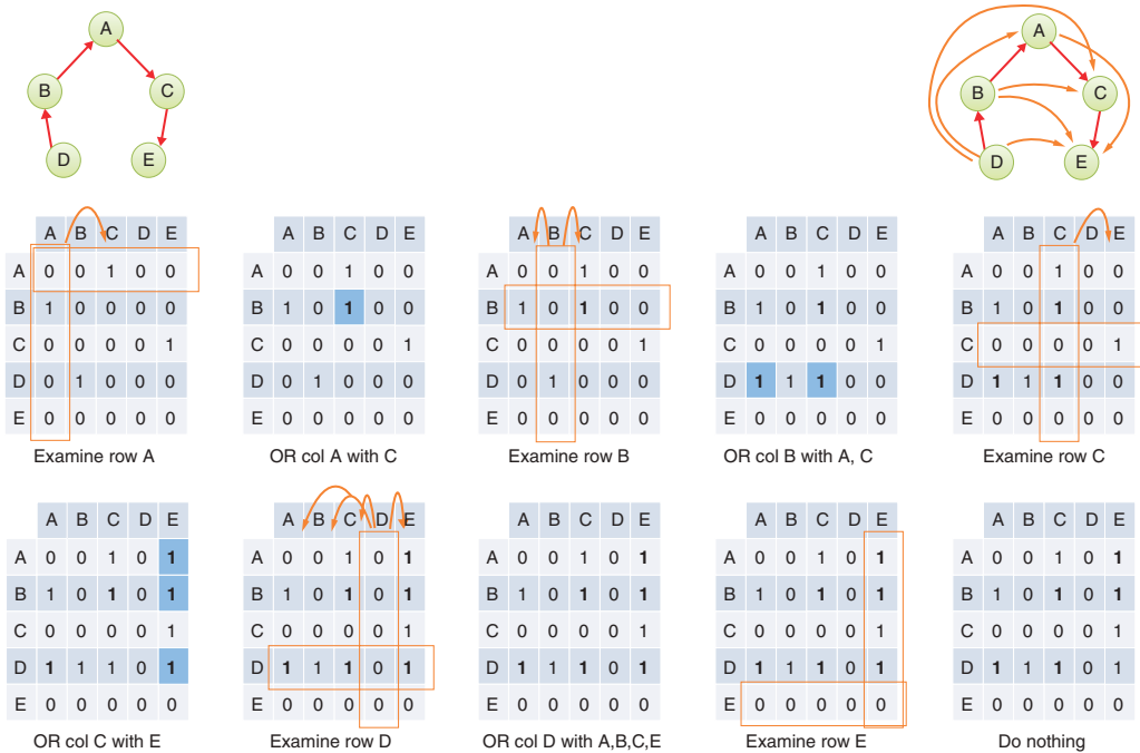
FIGURE 14-23 Marshall's algorithm on a long path
