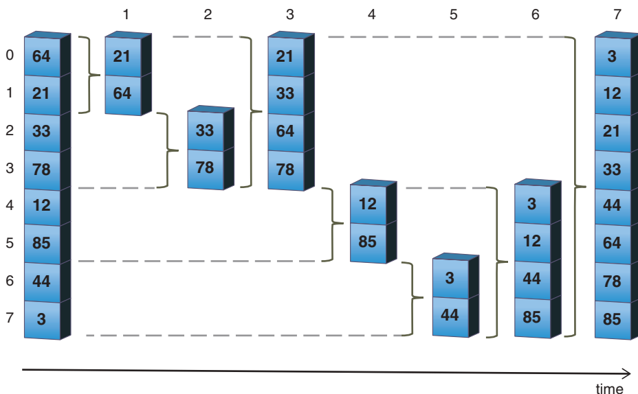
FIGURE 6-16 Mergesorting an eight-element array Humble Bundle Pearson Python Bundle – © Pearson. Do Not Distribute.
