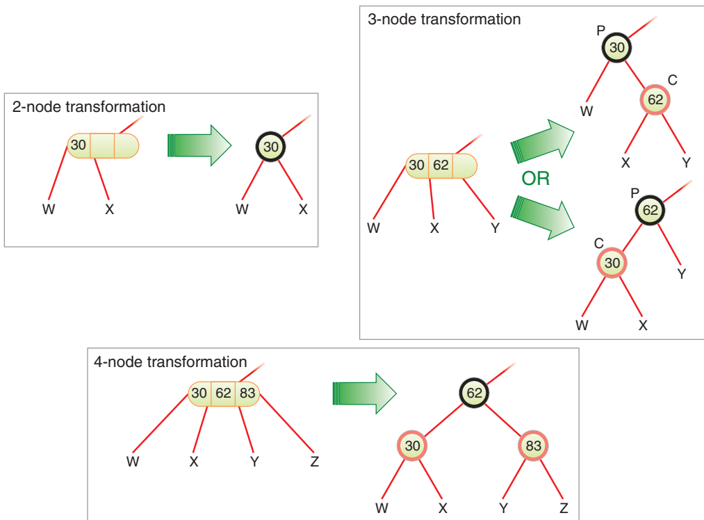
FIGURE 10-32 Transforming nodes: 2-3-4 to red-black
