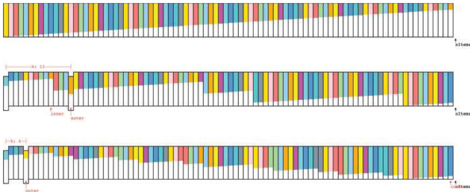
FIGURE 7-4 After the 40-sort and 13-sort in a 90-cell array
