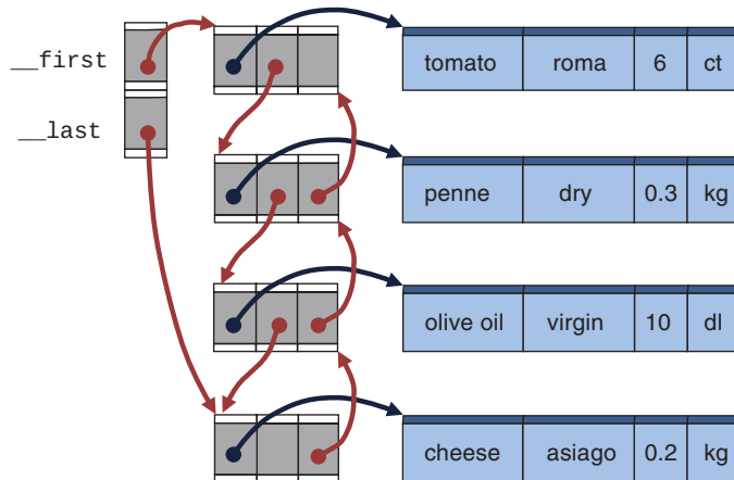
FIGURE 5-10 A doubly linked (and double-ended) list
