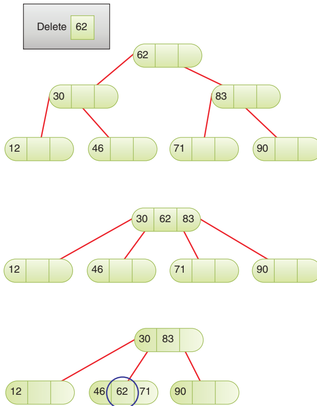
FIGURE 9-14 Deleting from a 2-3-4 tree with only 2-nodes
