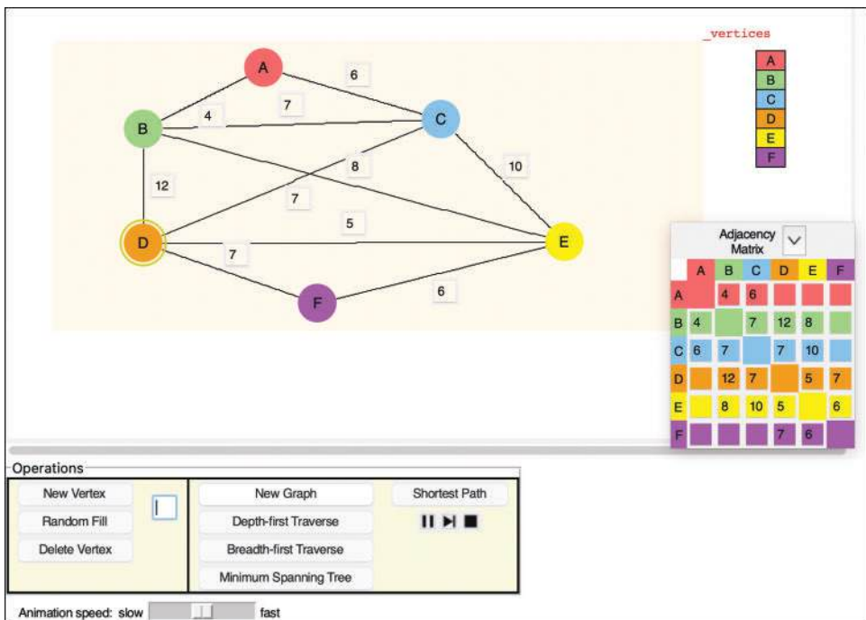
FIGURE 15-2 The WeightedGraph Visualization tool
