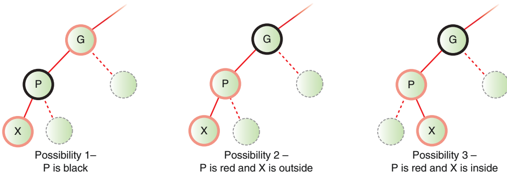
FIGURE 10-25 Three post-insertion possibilities
