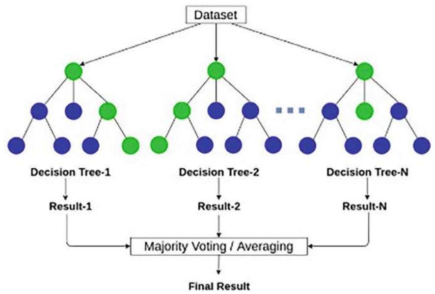
Fig. 2 Random forest
