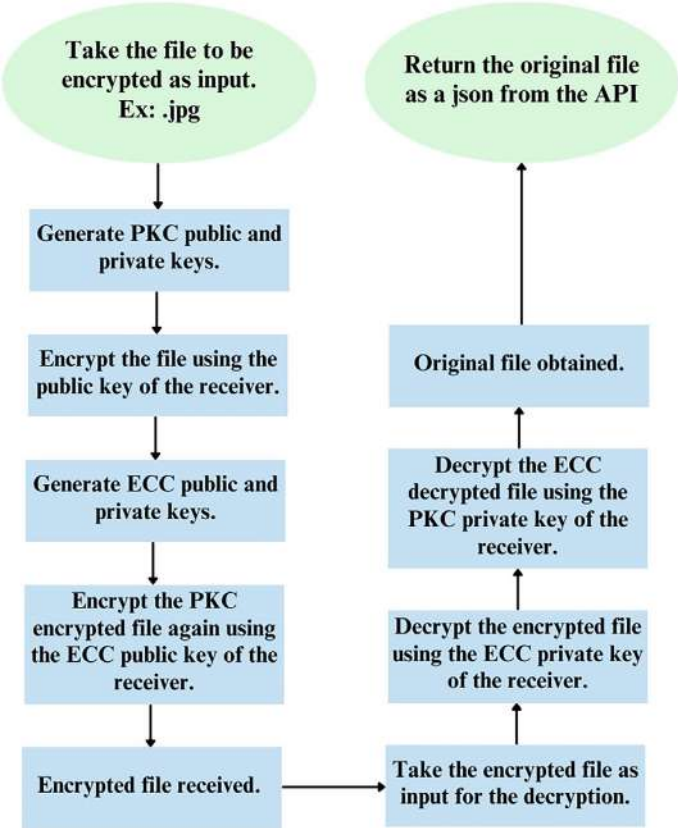
Fig. 5 Flowchart of encryption and decryption
