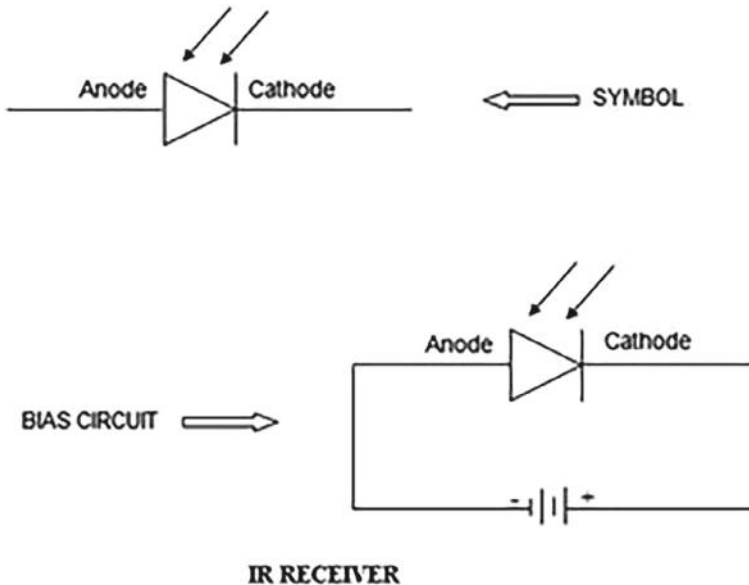
Fig. 5 IR receiver
