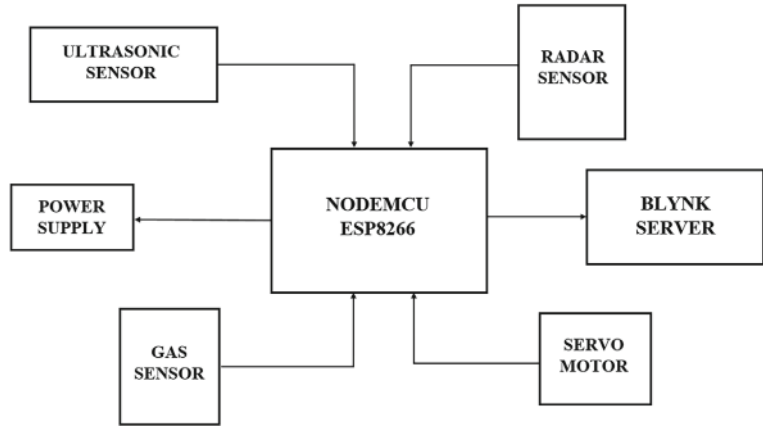
Fig. 9 Block diagram
