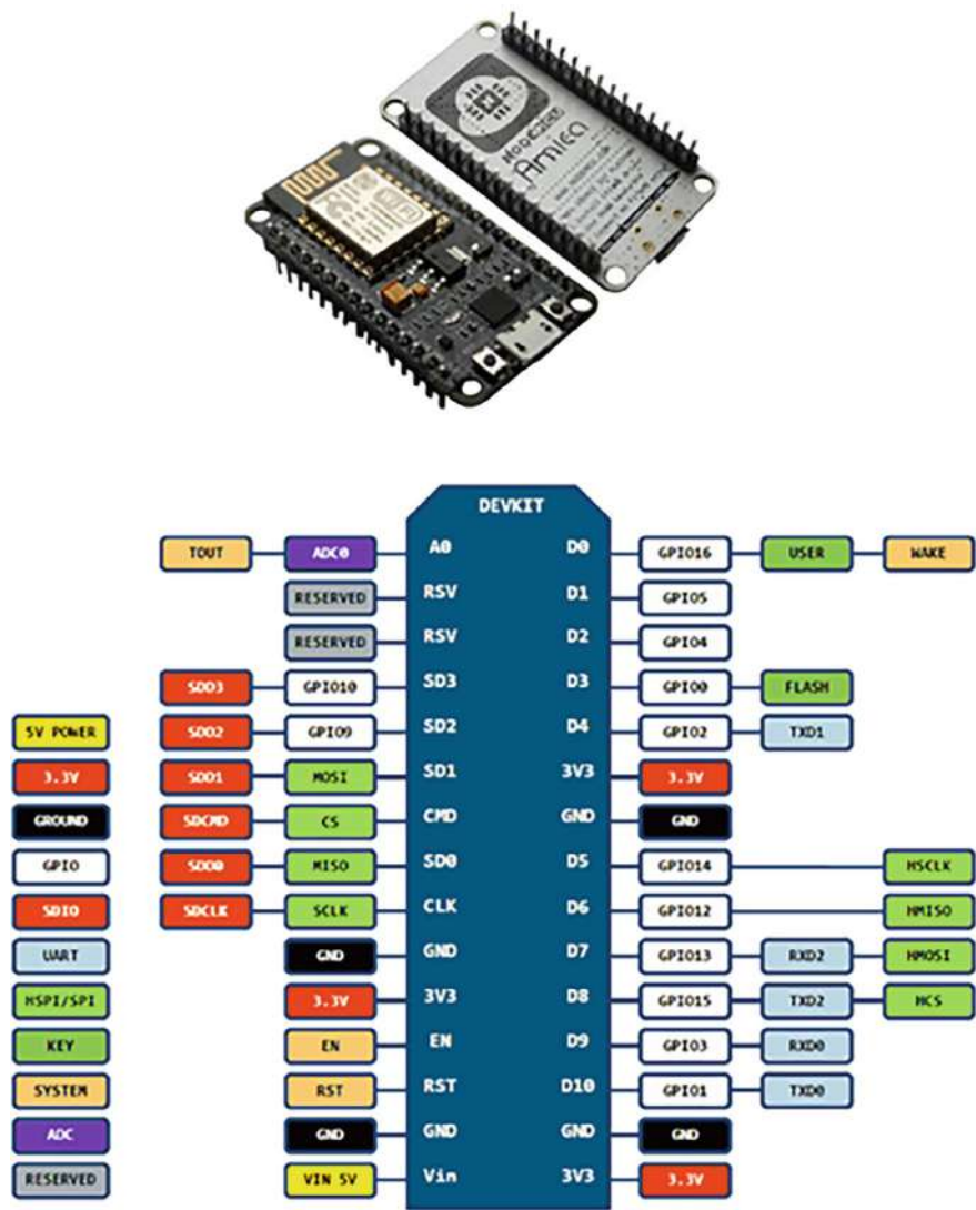
Fig. 1 ESP 12 chip and its pin diagram [18]
