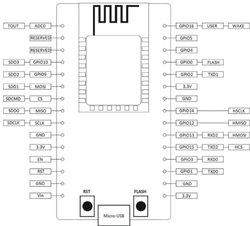
Fig. 2 Pins of node MCU
