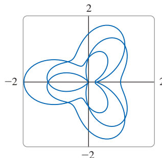
FIGURE 16 r = \sin^2(3\theta/2) + \cos^2(2\theta/3)
