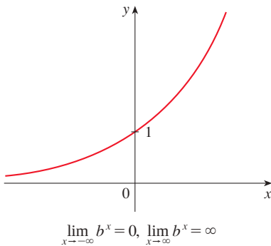
FIGURE 8 y = b^x , b > 1
