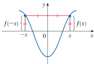
FIGURE 19 An even function
