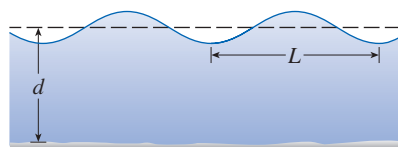
FIGURE 5 Idealized water wave
