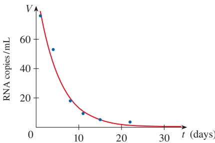
FIGURE 11 Exponential model for viral load
