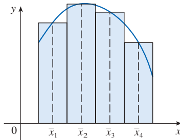
FIGURE 2 Midpoint approximation
