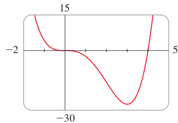
FIGURE 12 y = x^4 - 4x^3
