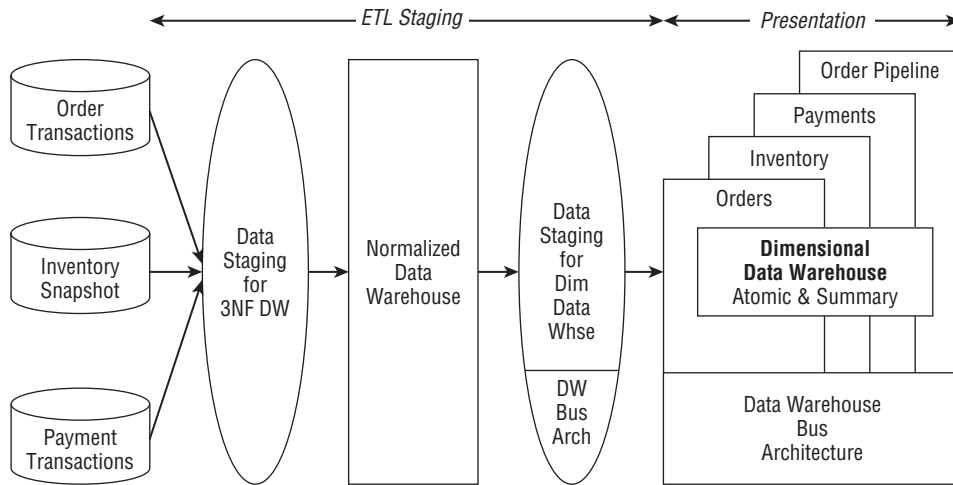
Figure 5-11: Hybrid of normalized data warehouse and dimensional data warehouse.
