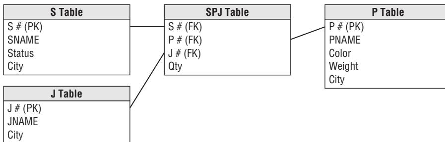
Figure 5-5: The suppliers and parts database.
