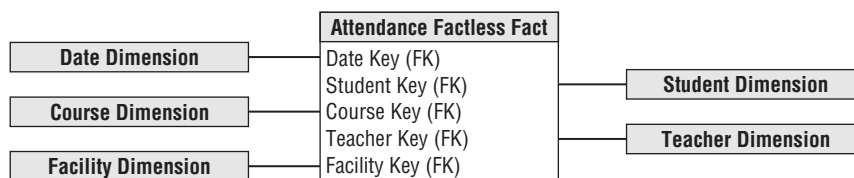
Figure 8-5: Daily student attendance is recorded in a factless fact table.
