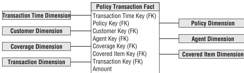
Figure 8-2: A transaction-grained insurance fact table.
