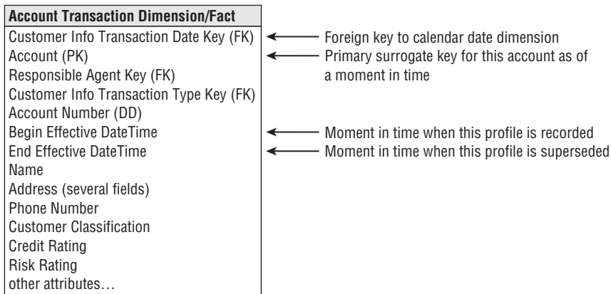
Figure 8-10: Fact table to capture customer information changes.
