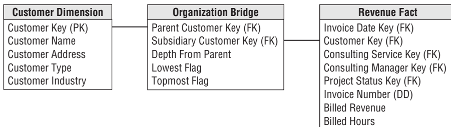
Figure 10-20: A bridge table between the fact and dimension table to navigate the organizational hierarchy.
