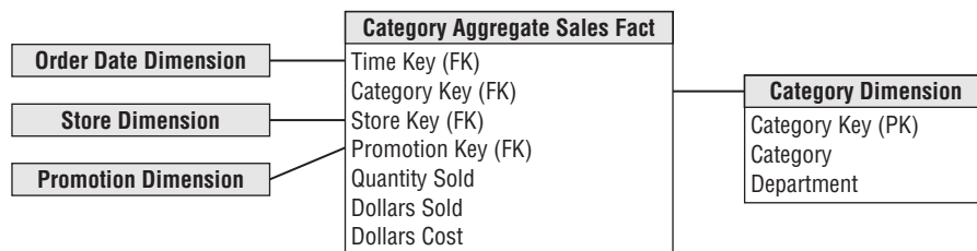
Figure 12-6: Aggregate records stored in separate fact and shrunken dimension tables is recommended.
