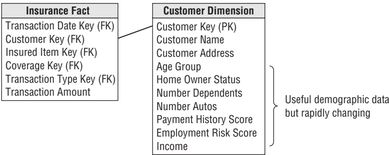
Figure 9-11: Customer dimension with rapidly changing demographic attributes.
