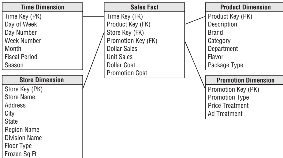
Figure 12-7: A base-level dimensional model.
