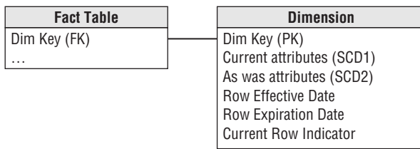
Figure 9-14: Tracking both “as was” and current profile attributes in a single dimension table.
