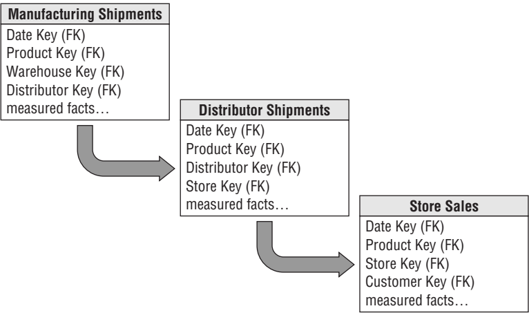
Figure 10-39: This value chain represents a product flow where each process is a fact table.
