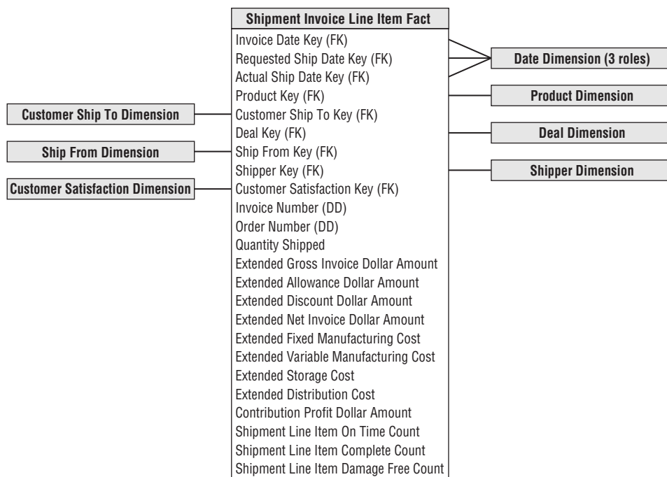
Figure 10-28: Treating satisfaction metrics as facts.
