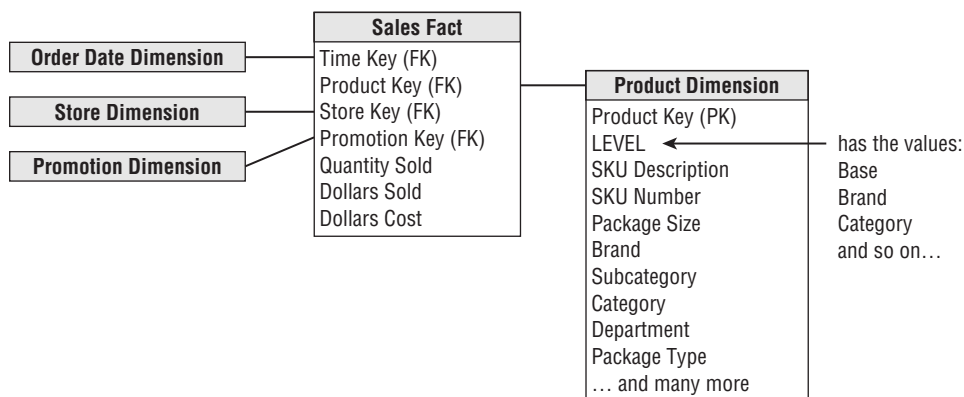
Figure 12-5: Aggregate records identified by the level attributes, which is not recommended.
