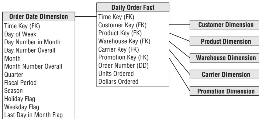
Figure 9-2: A basic dimensional design for order tracking.
