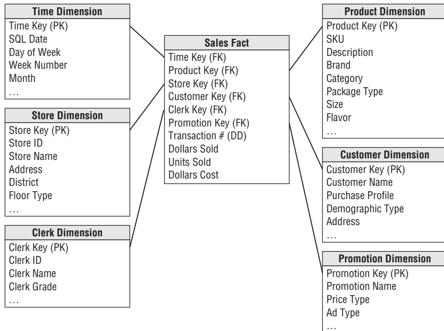
Figure 9-1: A sample data warehouse schema.
