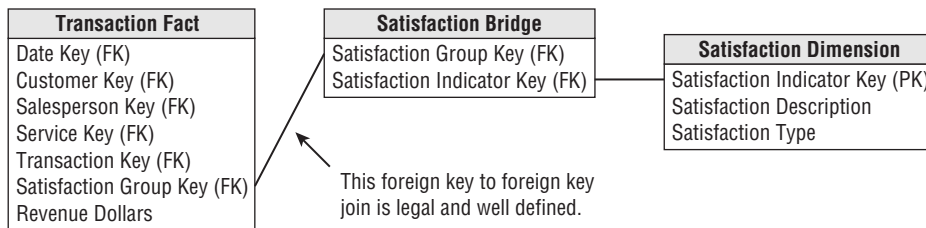
Figure 10-29: Using a bridge table between the transaction fact table and a satisfaction dimension.
