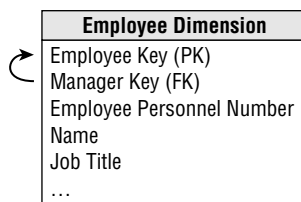
Figure 10-21: Basic structure of the employee dimension and reports-to hierarchy.
