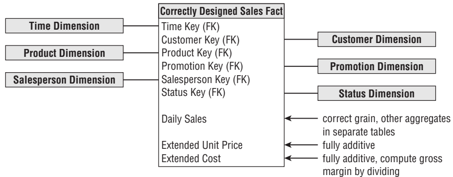
Figure 7-4: An example of a “good” fact table addressing the issues in Figure 7-3.
