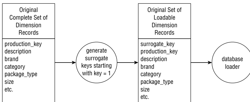
Figure 11-10: The original loading of a dimension where surrogate keys are assigned sequentially to every input record and the natural key becomes an ordinary attribute.
