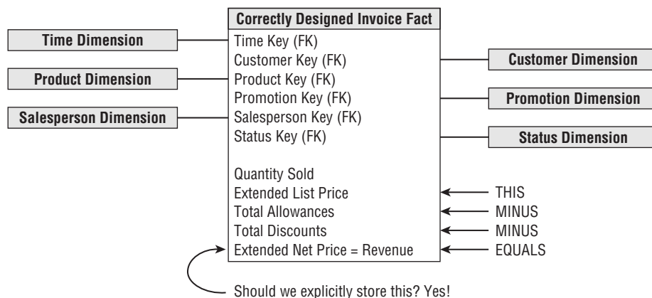
Figure 7-5: A customer billing fact table.
