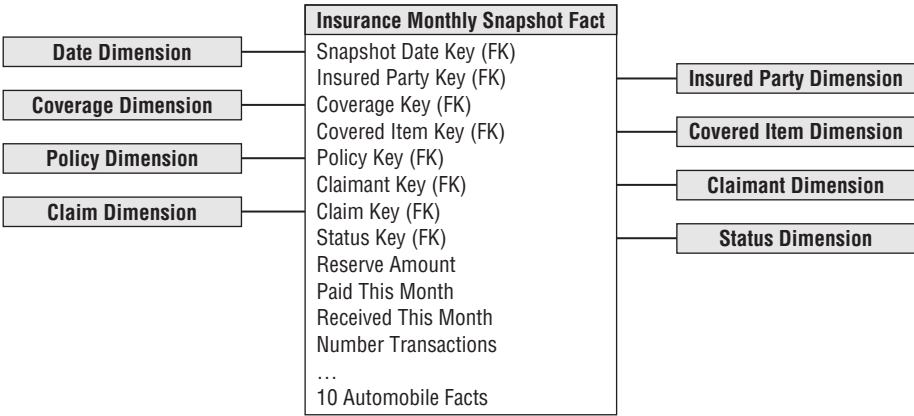
Figure 10-36: Monthly snapshot for automobile coverages.
