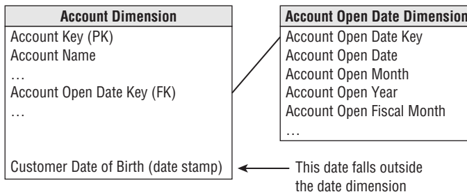
Figure 9-4: A dimension table with a date foreign key, as well as a date stamp attribute.
