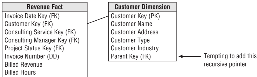
Figure 10-18: A fact table whose grain is the individual invoice line item.
