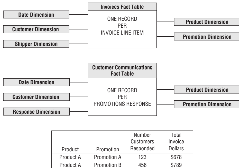
Figure 7-2: Two subject areas with conformed dimensions.
