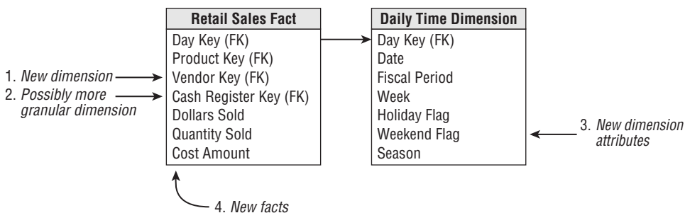
Figure 6-6: Potential changes to an existing dimensional model.
