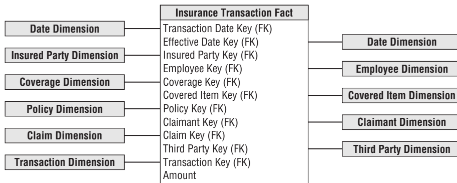
Figure 10-33: A claims transaction dimensional model.
