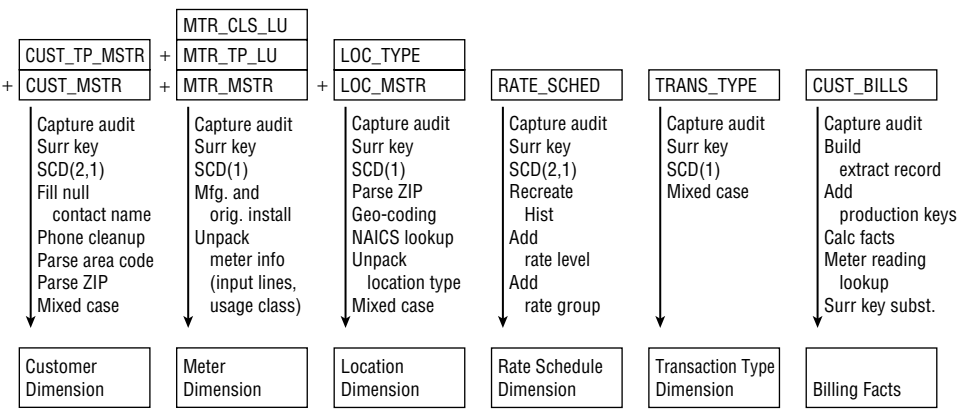
Figure 11-1: Simplified conceptual ETL plan.
