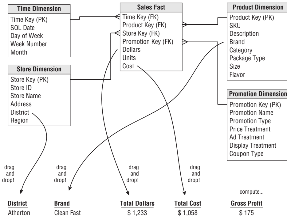
Figure 6-2: Dragging dimension attributes and facts into a report.
