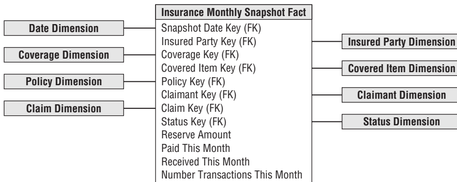
Figure 10-34: A claims monthly snapshot dimensional model.
