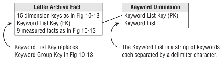
Figure 10-14: The same fact table showing the keyword dimension containing a variable-length text string keyword list.
