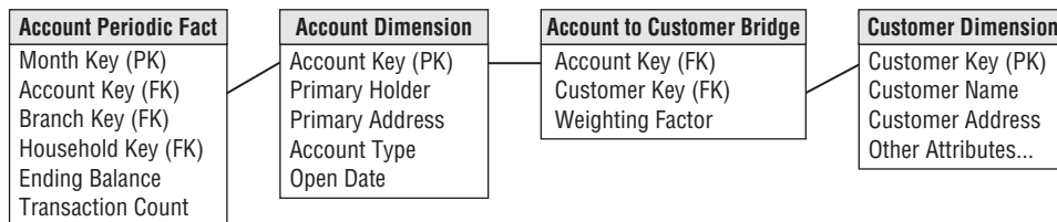
Figure 10-3: A bridge table resolves a many-valued dimension attribute.
