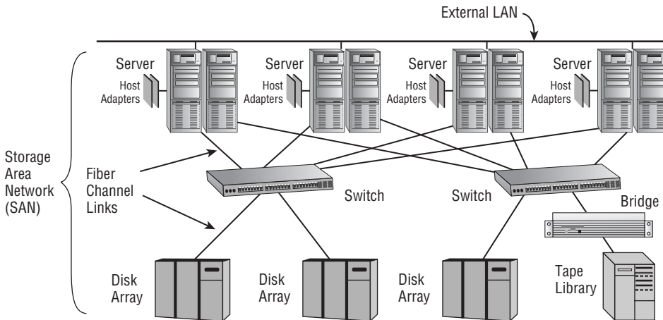
Figure 12-10: A typical storage area network configuration.
