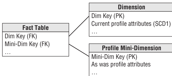
Figure 9-13: A mini-dimension for capturing profile changes with type 1 overwrite in the primary dimension table.
