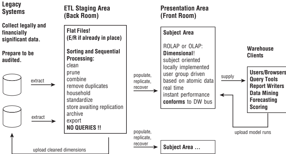
Figure 2-3: The enterprise data warehouse, showing the back room ETL staging area and the front room presentation area.
