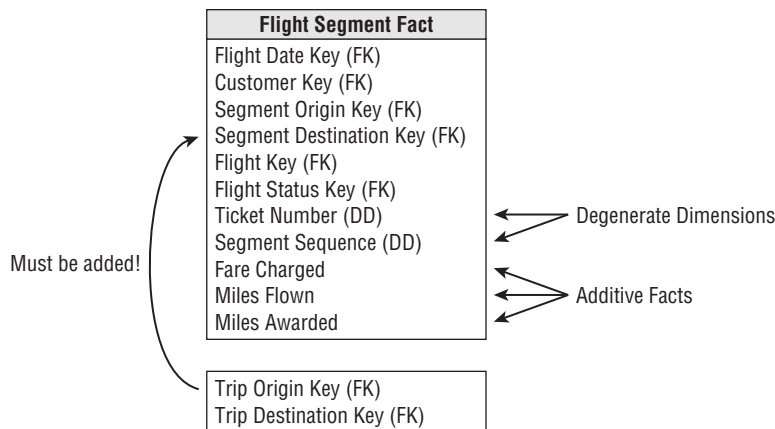
Figure 10-37: The flight segment dimensional model.
