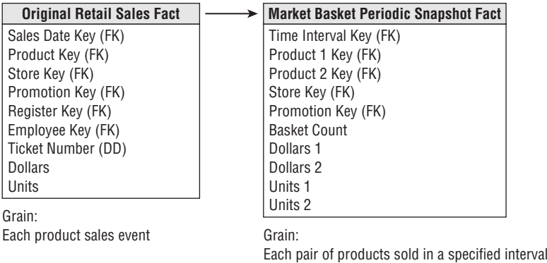
Figure 10-43: A market basket fact table based on atomic retail sales data.
