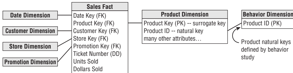
Figure 13-13: A special behavior dimension is added to a normal dimensional model to restrict the schema to the context of a behaviorally defined group of products.
