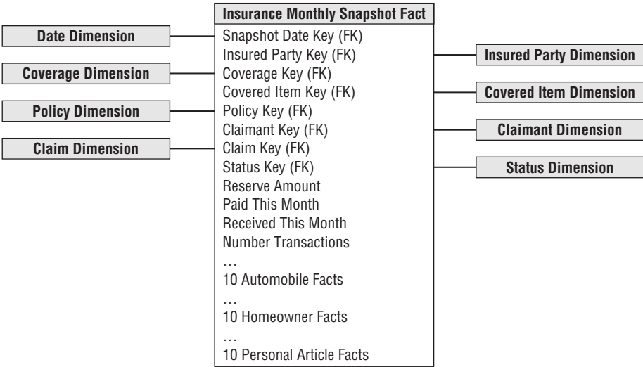
Figure 10-35: Inappropriate way to handle the facts unique to each line of business.
