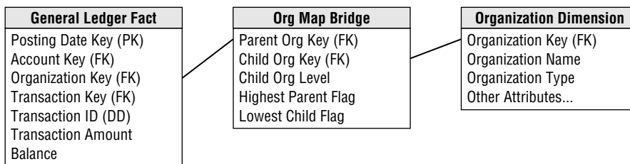
Figure 10-4: A bridge table models a hierarchical variable-depth relationship.
