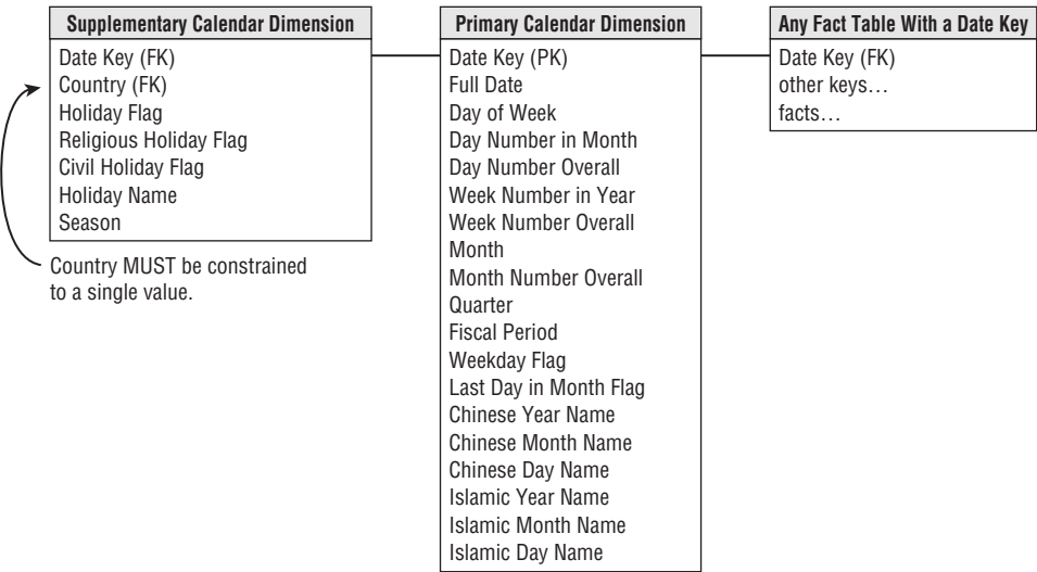
Figure 10-31: Primary and supplementary calendar dimensions for organizations that must track multiple national calendars.
