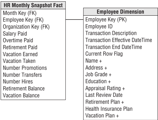
Figure 10-38: A human resources monthly snapshot with a type 2 slowly changing employee dimension table.
