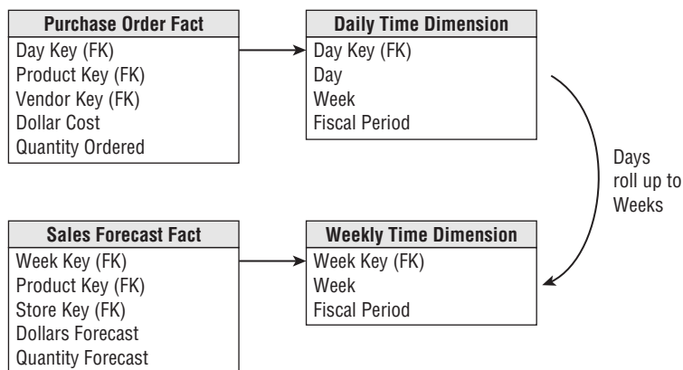
Figure 6-5: Two fact tables with conformed dimensions.
