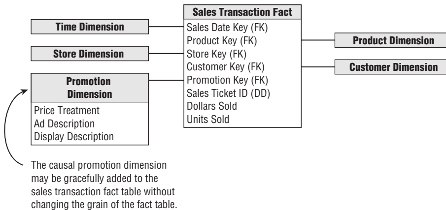
Figure 9-10: A typical dimensional schema for a set of retail sales transactions with a “causal” promotion dimension.
