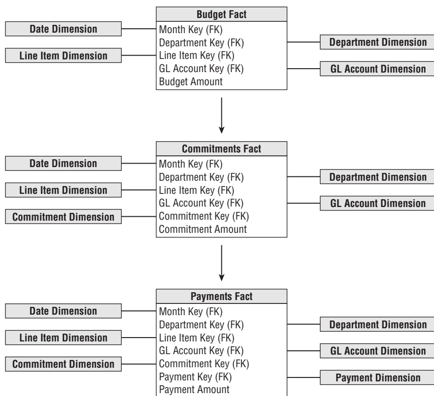
Figure 10-40: The budget chain showing the budget, commitments, and payments fact tables.
