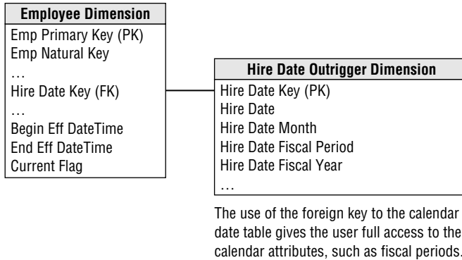
Figure 10-2: A date dimension outrigger joined to the employee dimension.
