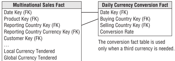
Figure 10-32: A fact table simultaneously recording sales in many different currencies. The currency conversion table is only used when converting to a third currency.
