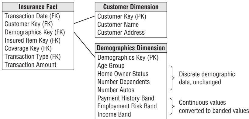
Figure 9-12: Separating frequently changing customer attributes in a demographics mini-dimension.
