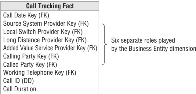
Figure 9-7: Multiple business entities associated with a phone call.
