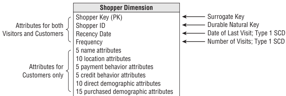
Figure 10-5: Shopper dimension with both visitor and customer attributes.
