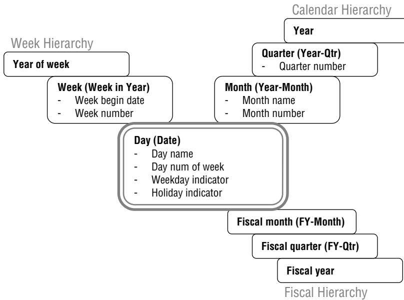
Figure 10-15: Graphical representation of multiple date hierarchies.
