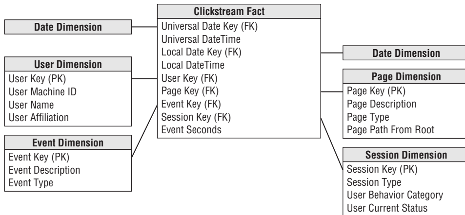
Figure 10-42: The dimensional model for clickstream events.
