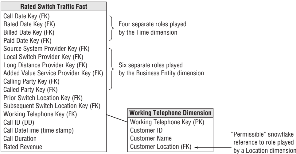
Figure 9-8: Sample schema with extensive role playing.
