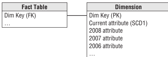
Figure 9-16: A dimension table with a series of type 3 attributes to track predictable changes.
