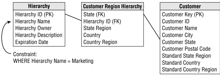
Figure 10-27: Using a bridge table to support multiple alternate hierarchies.
