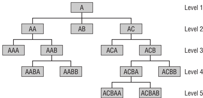
Figure 10-26: Sample org chart with pathstring values.
