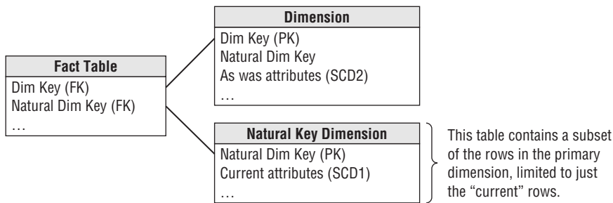
Figure 9-15: One foreign key in the fact table joins to a SCD2 dimension table, while the natural/durable key joins to only the most current version of the dimension.
