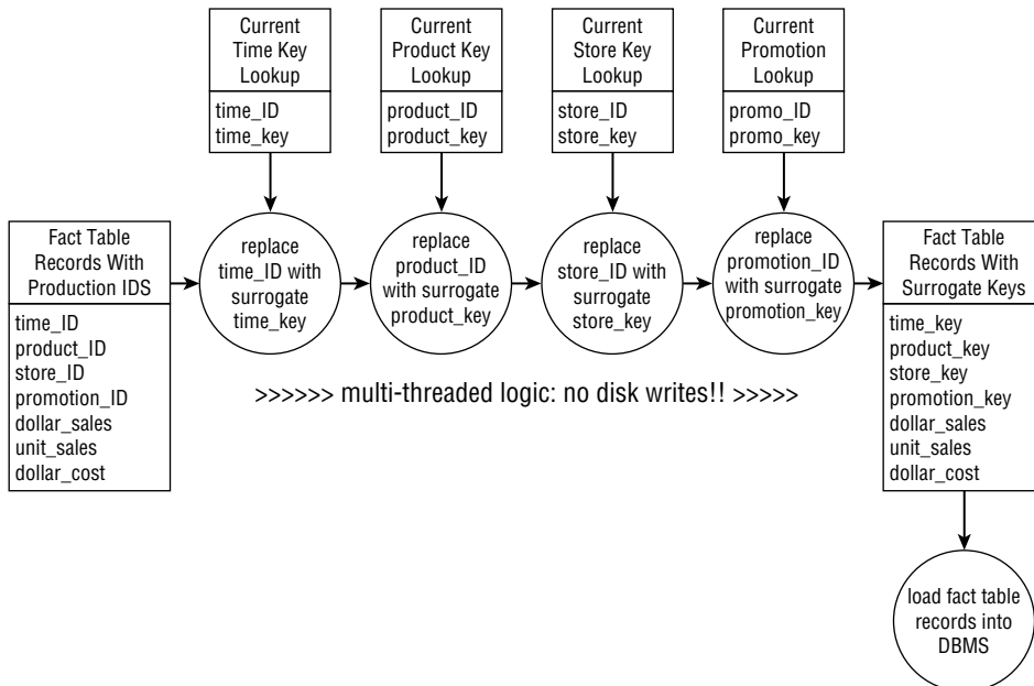
Figure 11-13: The pipelined fact table processing logic for replacing all natural keys (designated as IDs) with surrogate keys.
