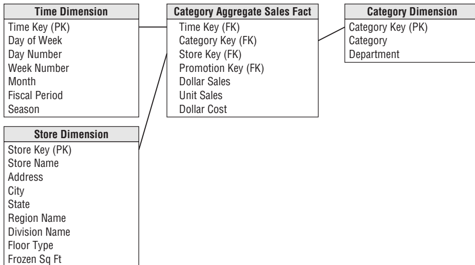
Figure 12-8: An aggregated dimensional schema derived from Figure 12-7 by aggregating to the category level.
