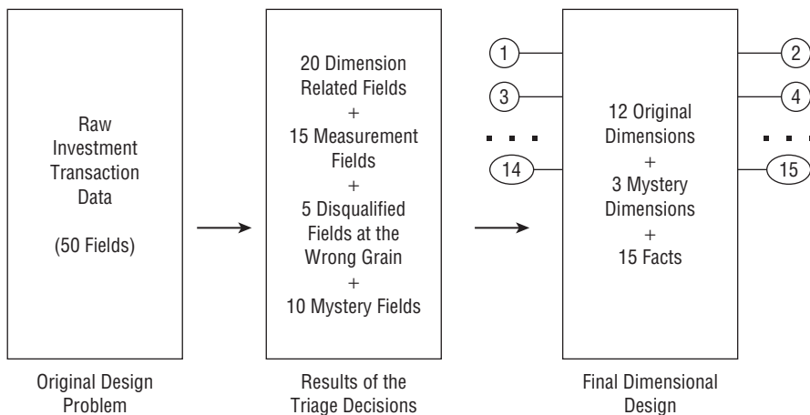
Figure 9-9: The logical progression of transforming complex source data into its corresponding dimensional model.
