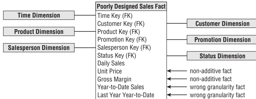
Figure 7-3: An example of a “bad” fact table.
