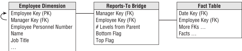
Figure 10-22: Classic relational structure for a reports-to hierarchy.
