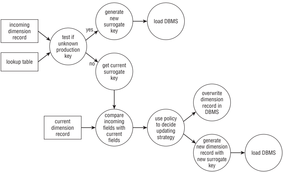
Figure 11-12: Dimension processing logic for all refreshes of a dimension table after the original load.
