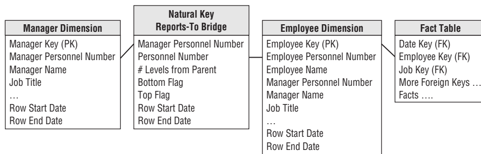
Figure 10-24: Tracking history in the reports-to relationship with a natural key bridge table.
