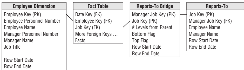
Figure 10-23: Separate employee and reports-to (or job) dimensions.
