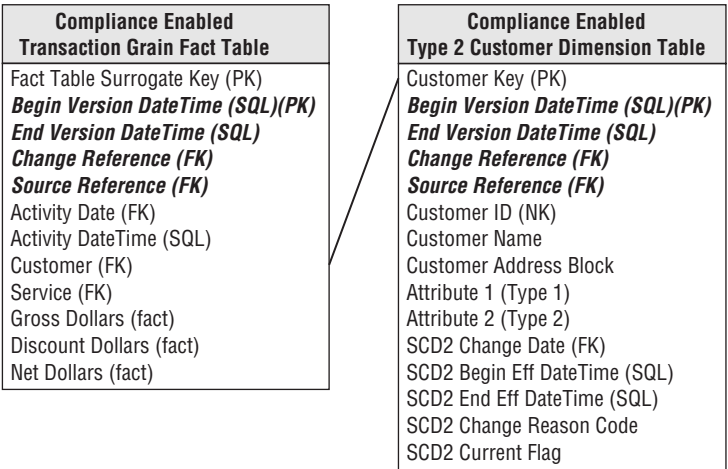
Figure 10-41: Compliance-enabled fact and dimension tables.
