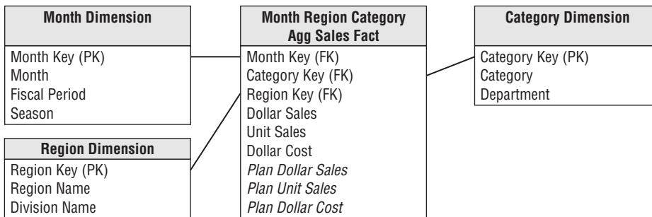
Figure 12-9: The three-way aggregate table formed by aggregating time to month, product to category, and store to region.
