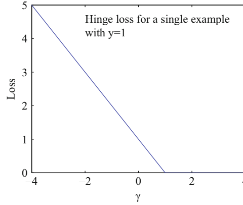
Figure 2.1: The hinge loss, plotted for the case y_i = 1 . The horizontal variable is the \gamma_i = \mathbf{a}^T \mathbf{x}_i + b of the text. Notice that giving a strong negative response to this positive example causes a loss that grows linearly as the magnitude of the response grows. Notice also that giving an insufficiently positive response also causes a loss. Giving a strongly positive response is free
