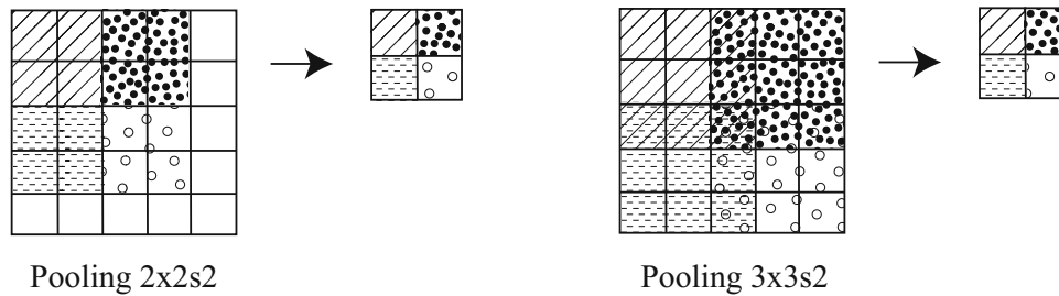
Figure 17.7: In a pooling layer, pooling units compute a summary of their inputs, then pass it on. The most common case is 2 \times 2 , illustrated here on the left . We tile each feature map with 2 \times 2 windows that do not overlap (so have stride 2). Pooling units compute a summary of the inputs (usually either the max or the average), then pass that on to the corresponding location in the corresponding feature map of the output block. As a result, the spatial dimensions of the output block will be about half those of the input block. On the right , the common alternative of pooling in overlapping 3 \times 3 windows with stride 2
