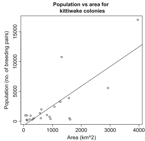
Figure 10.20: A regression of the number of breeding pairs of kittiwakes against the area of an island, for 22 data points
