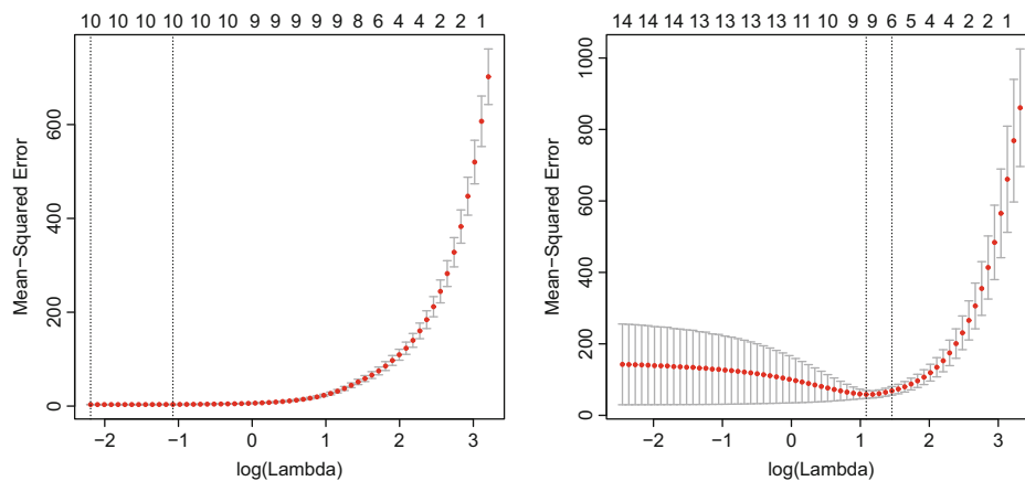
Figure 11.4: Plots of mean-squared error as a function of log regularization parameter (i.e., \log \lambda ) for a regression of weight against all variables for the bodyfat dataset using an L_1 regularizer (i.e., a lasso). These plots show mean-squared error averaged over cross-validation folds with a vertical one standard deviation bar. On the left , the plot for the dataset with the six outliers identified in Fig. 10.15 removed. On the right , the plot for the whole dataset. Notice how the outliers increase the variability of the error, and the best error. The top row of numbers gives the number of non-zero components in \hat{\beta} . Notice how as \lambda increases, this number falls (there are 15 explanatory variables, so the largest model would have 15 variables). The penalty ensures that explanatory variables with small coefficients are dropped as \lambda gets bigger
