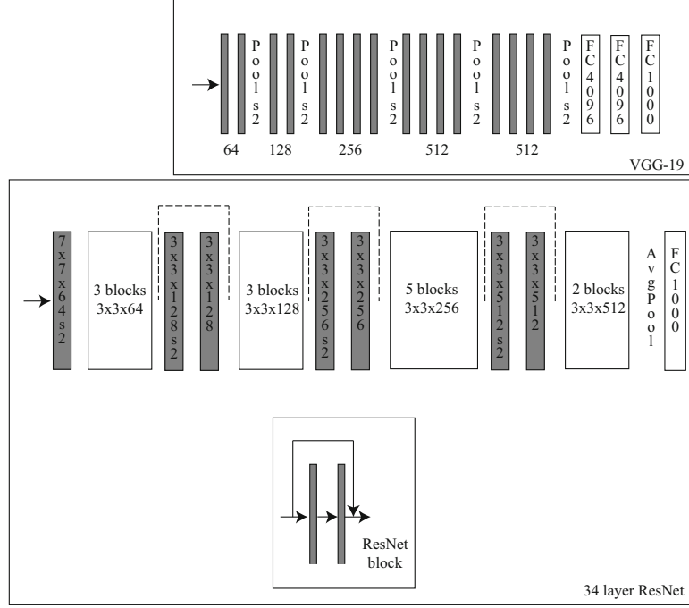
Figure 18.5: Comparing VGG-19 to a 34 layer ResNet requires an even more compact graphical representation. Each shaded box is a convolutional layer of 3 \times 3 \times D kernels followed by a ReLU. The number of kernels is given the notation below the box, and D follows by matching sizes. Every layer with learnable parameters is represented by a box, so VGG-19 has 19 such layers, together with pooling layers. The 34 layer ResNet has 34 such layers. There are a few specialized layers (text in the box), but most appear in the blocks (inset) which have two 3 \times 3 \times D layers with a residual connection that skips both. These blocks are stacked, as indicated in the figure. The dashed lines around greyed blocks represent a residual connection that causes the size of the data block to change
