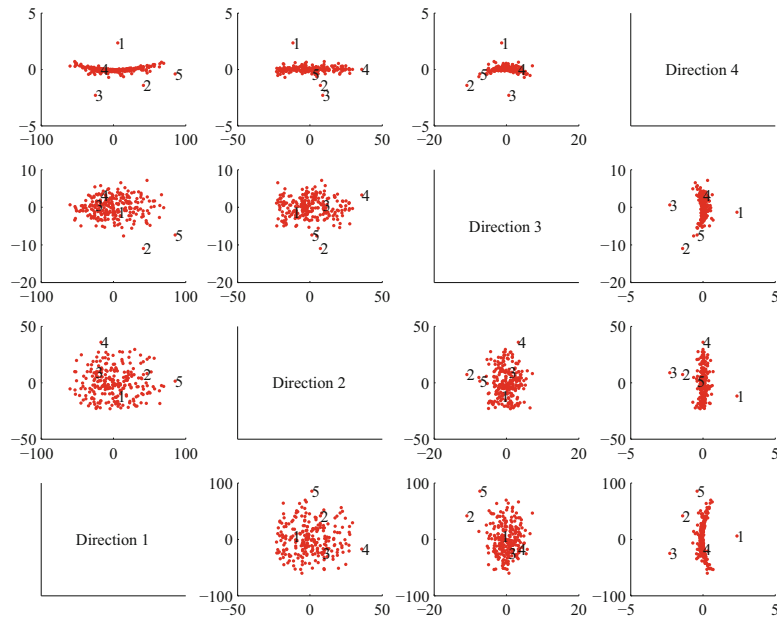
Figure 5.3: A panel plot of the bodyfat dataset of Fig. 4.4, now rotated so that the covariance between all pairs of distinct dimensions is zero. Now we do not know names for the directions—they’re linear combinations of the original variables. Compare this figure with Fig. 5.2; in that figure, the axes were the same, but in this figure I have scaled the axes so you can see details. Notice that the blob is a little curved, and there are several data points that seem to lie some way away from the blob, which I have numbered
