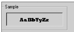
Figure 7.90: Sample box.
