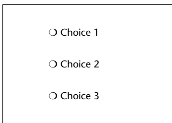
Figure 4.1: Single menu.
